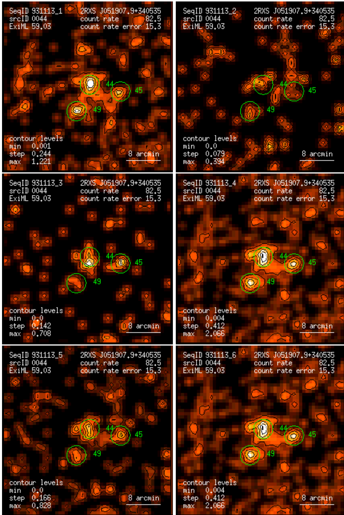
Figure 44: RASS 931113: detection 0044: band rate images, Gaussian filter: (1) PSPC channels 11 – 41, (2) 52 – 90, (3) 91 – 201, (4) 11 – 235, (5) 52 – 201, (6) 11 – 201. Broad band rates in counts/ks. Band rate contour levels in counts/ks/arcmin 2 .
