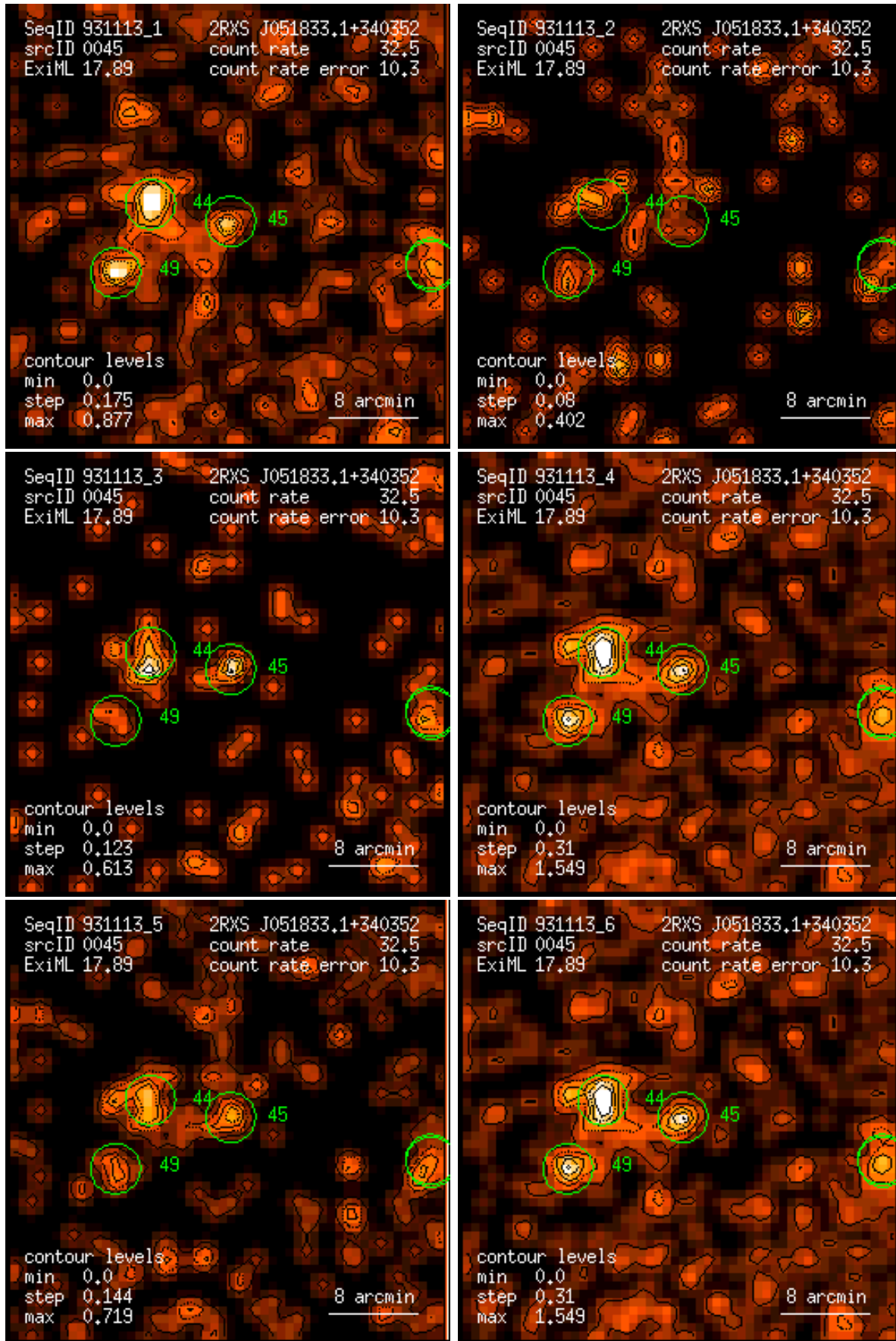
Figure 45: RASS 931113: detection 0045: band rate images, Gaussian filter: (1) PSPC channels 11 – 41, (2) 52 – 90, (3) 91 – 201, (4) 11 – 235, (5) 52 – 201, (6) 11 – 201. Broad band rates in counts/ks. Band rate contour levels in counts/ks/arcmin 2 .
