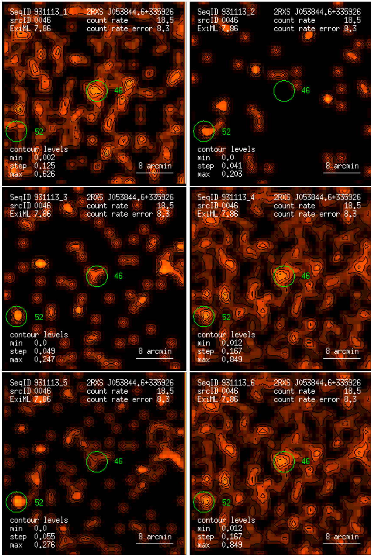
Figure 46: RASS 931113: detection 0046: band rate images, Gaussian filter: (1) PSPC channels 11 – 41, (2) 52 – 90, (3) 91 – 201, (4) 11 – 235, (5) 52 – 201, (6) 11 – 201. Broad band rates in counts/ks. Band rate contour levels in counts/ks/arcmin 2 .
