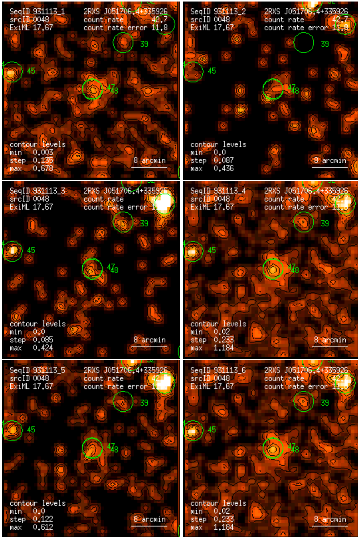
Figure 48: RASS 931113: detection 0048: band rate images, Gaussian filter: (1) PSPC channels 11 – 41, (2) 52 – 90, (3) 91 – 201, (4) 11 – 235, (5) 52 – 201, (6) 11 – 201. Broad band rates in counts/ks. Band rate contour levels in counts/ks/arcmin 2 .
