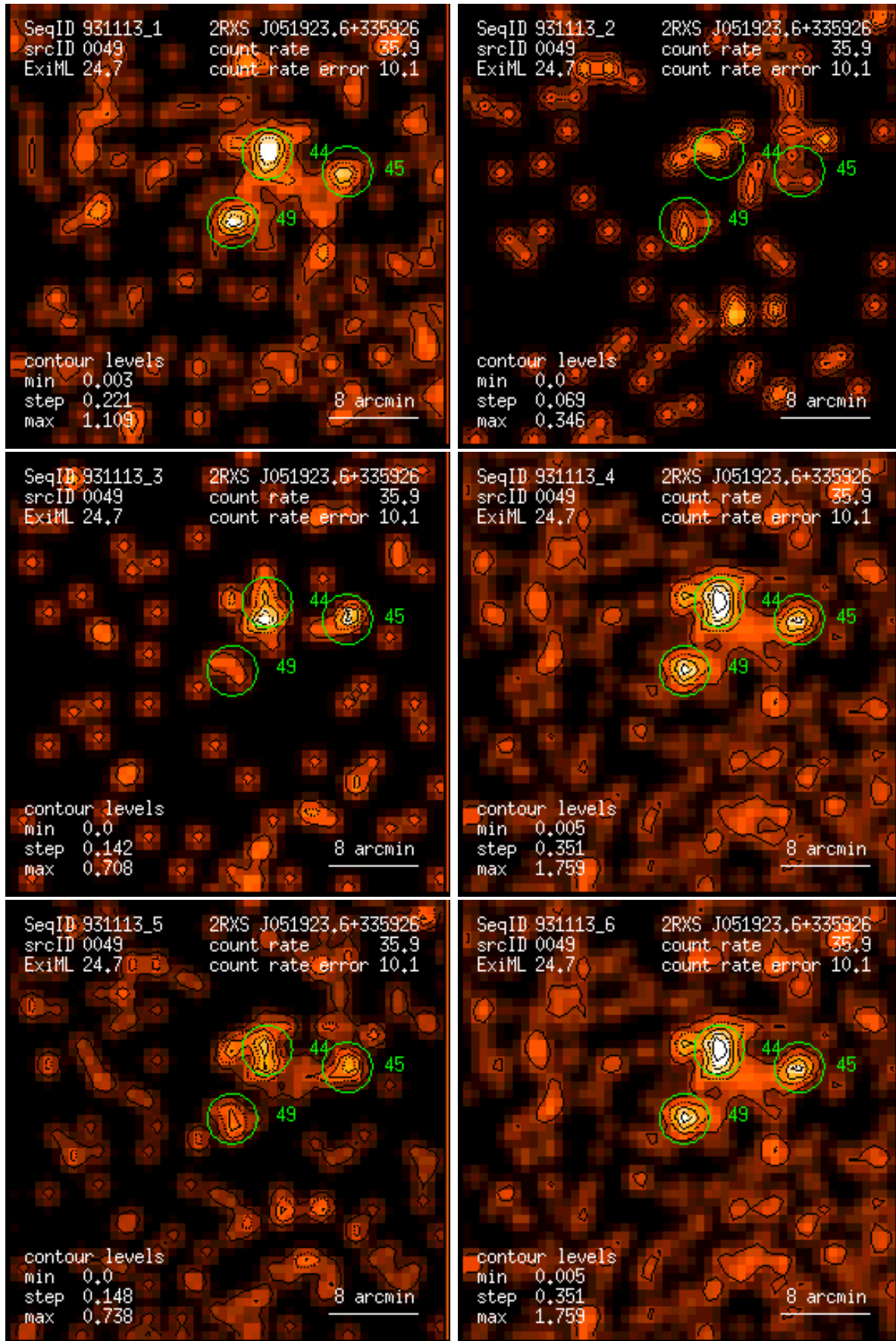
Figure 49: RASS 931113: detection 0049: band rate images, Gaussian filter: (1) PSPC channels 11 – 41, (2) 52 – 90, (3) 91 – 201, (4) 11 – 235, (5) 52 – 201, (6) 11 – 201. Broad band rates in counts/ks. Band rate contour levels in counts/ks/arcmin 2 .
