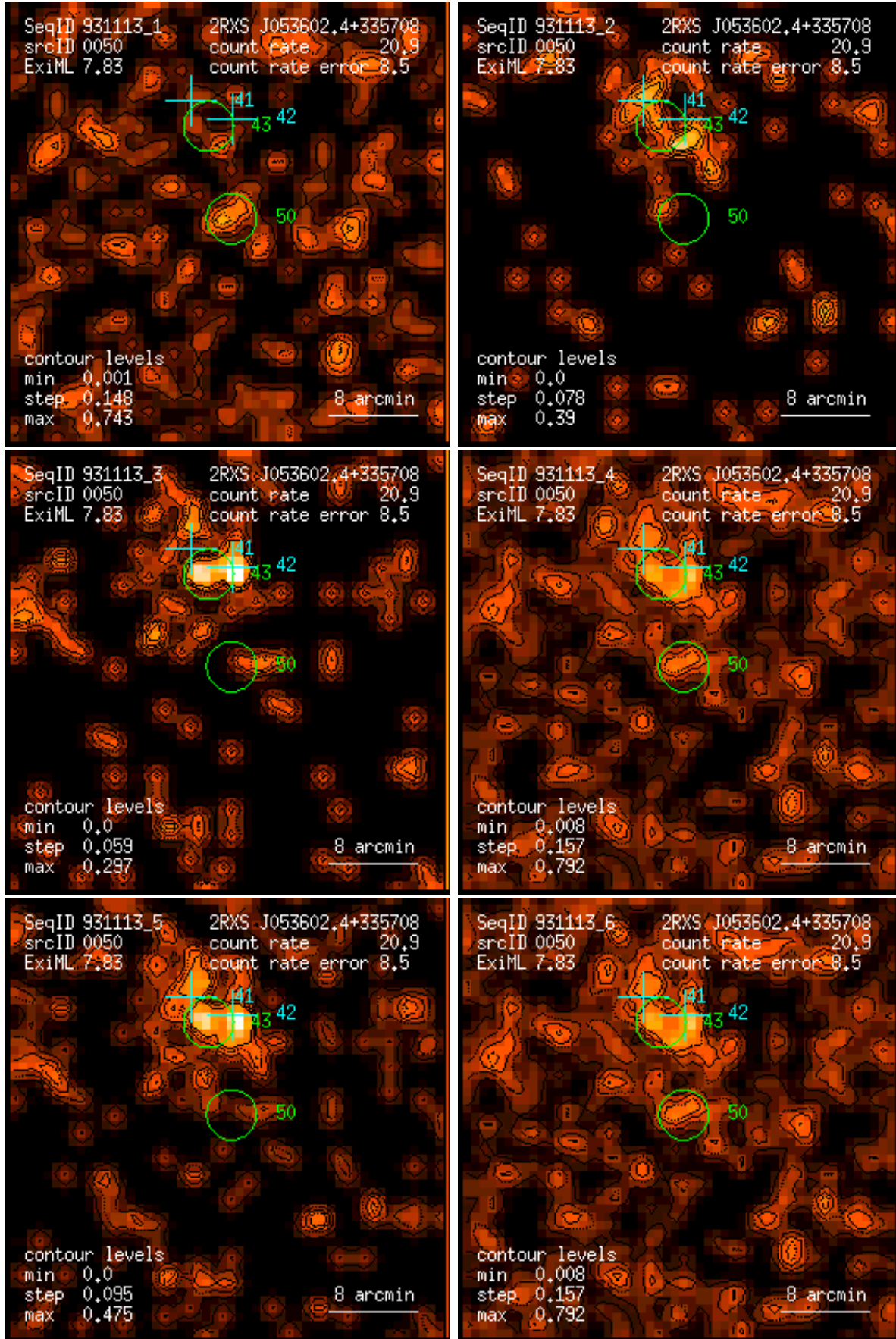
Figure 50: RASS 931113: detection 0050: band rate images, Gaussian filter: (1) PSPC channels 11 – 41, (2) 52 – 90, (3) 91 – 201, (4) 11 – 235, (5) 52 – 201, (6) 11 – 201. Broad band rates in counts/ks. Band rate contour levels in counts/ks/arcmin 2 .
