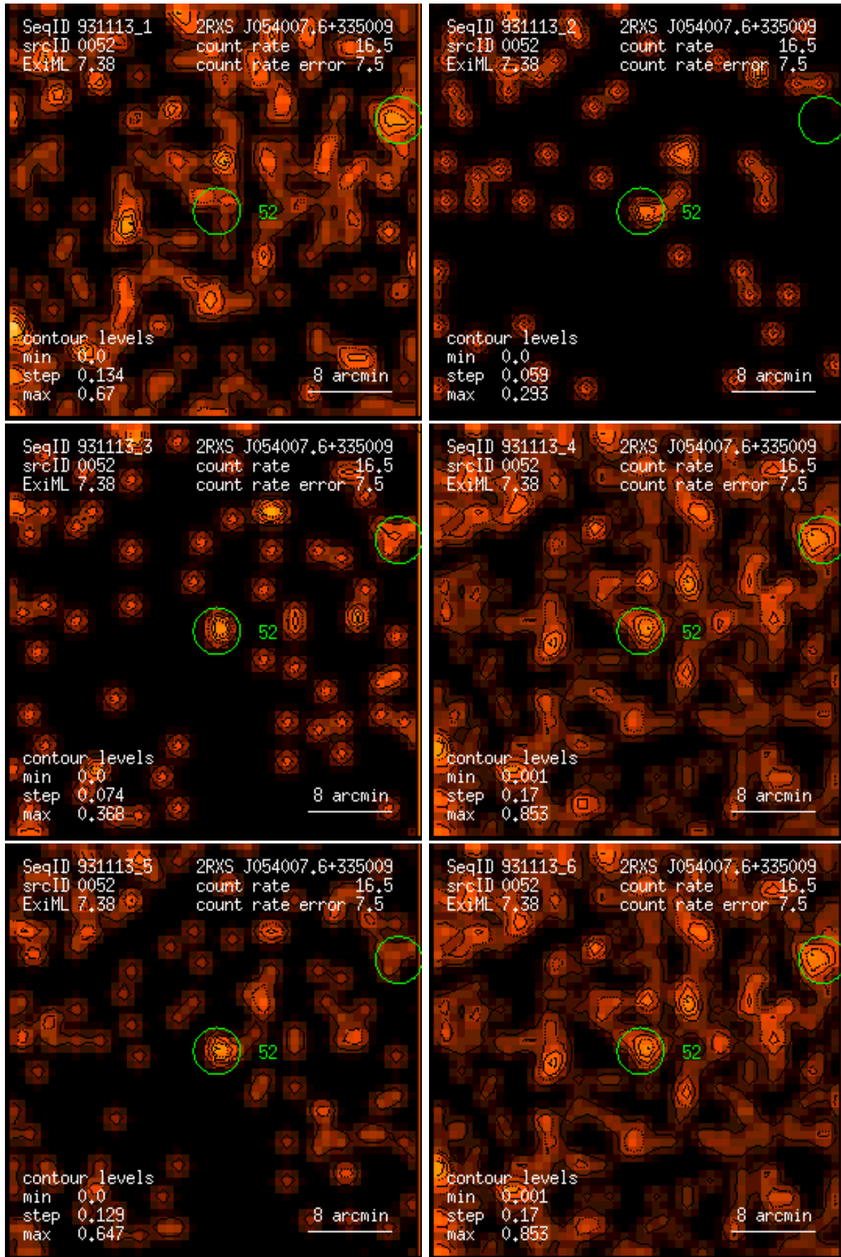
Figure 52: RASS 931113: detection 0052: band rate images, Gaussian filter: (1) PSPC channels 11 – 41, (2) 52 – 90, (3) 91 – 201, (4) 11 – 235, (5) 52 – 201, (6) 11 – 201. Broad band rates in counts/ks. Band rate contour levels in counts/ks/arcmin 2 .
