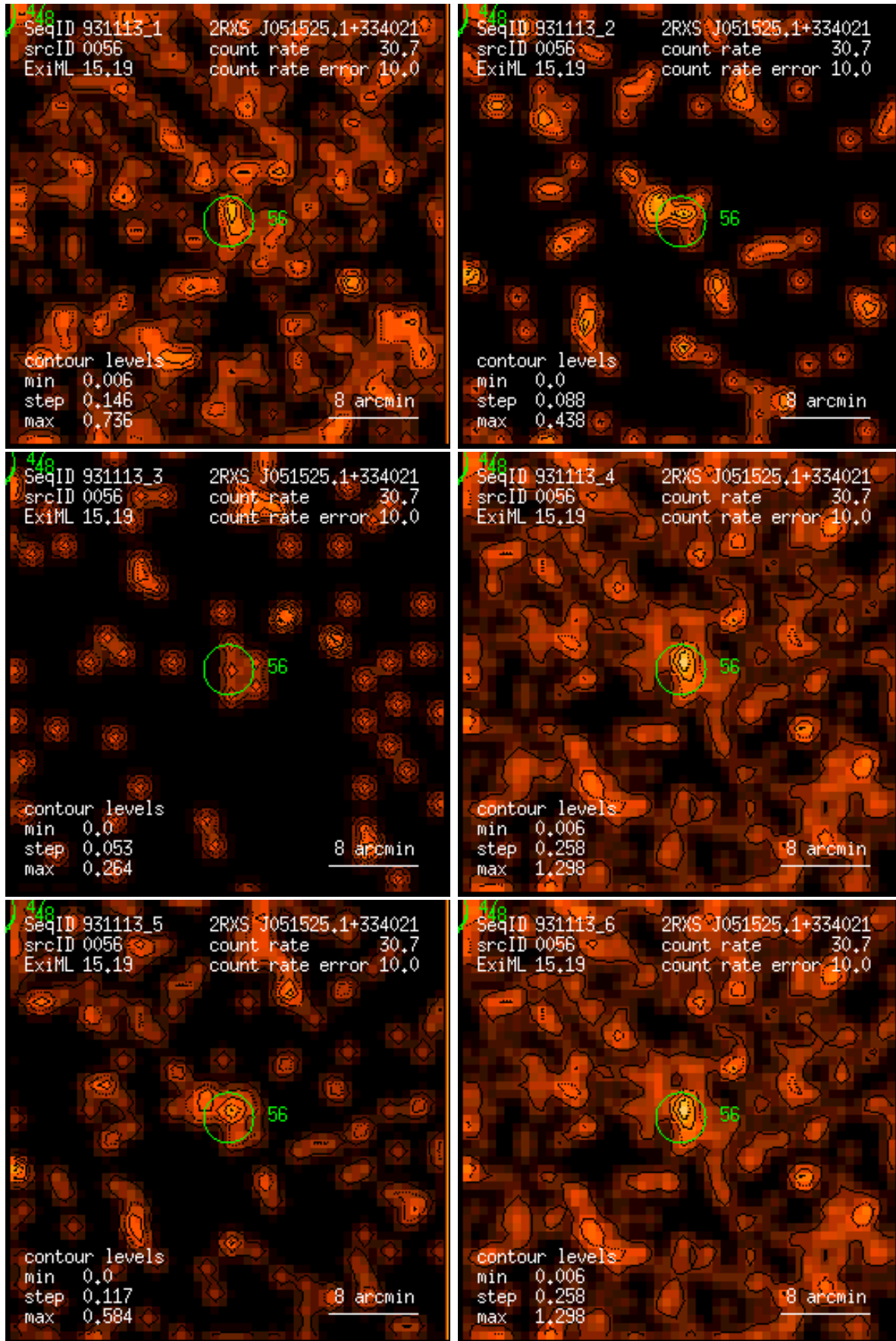
Figure 56: RASS 931113: detection 0056: band rate images, Gaussian filter: (1) PSPC channels 11 – 41, (2) 52 – 90, (3) 91 – 201, (4) 11 – 235, (5) 52 – 201, (6) 11 – 201. Broad band rates in counts/ks. Band rate contour levels in counts/ks/arcmin 2 .
