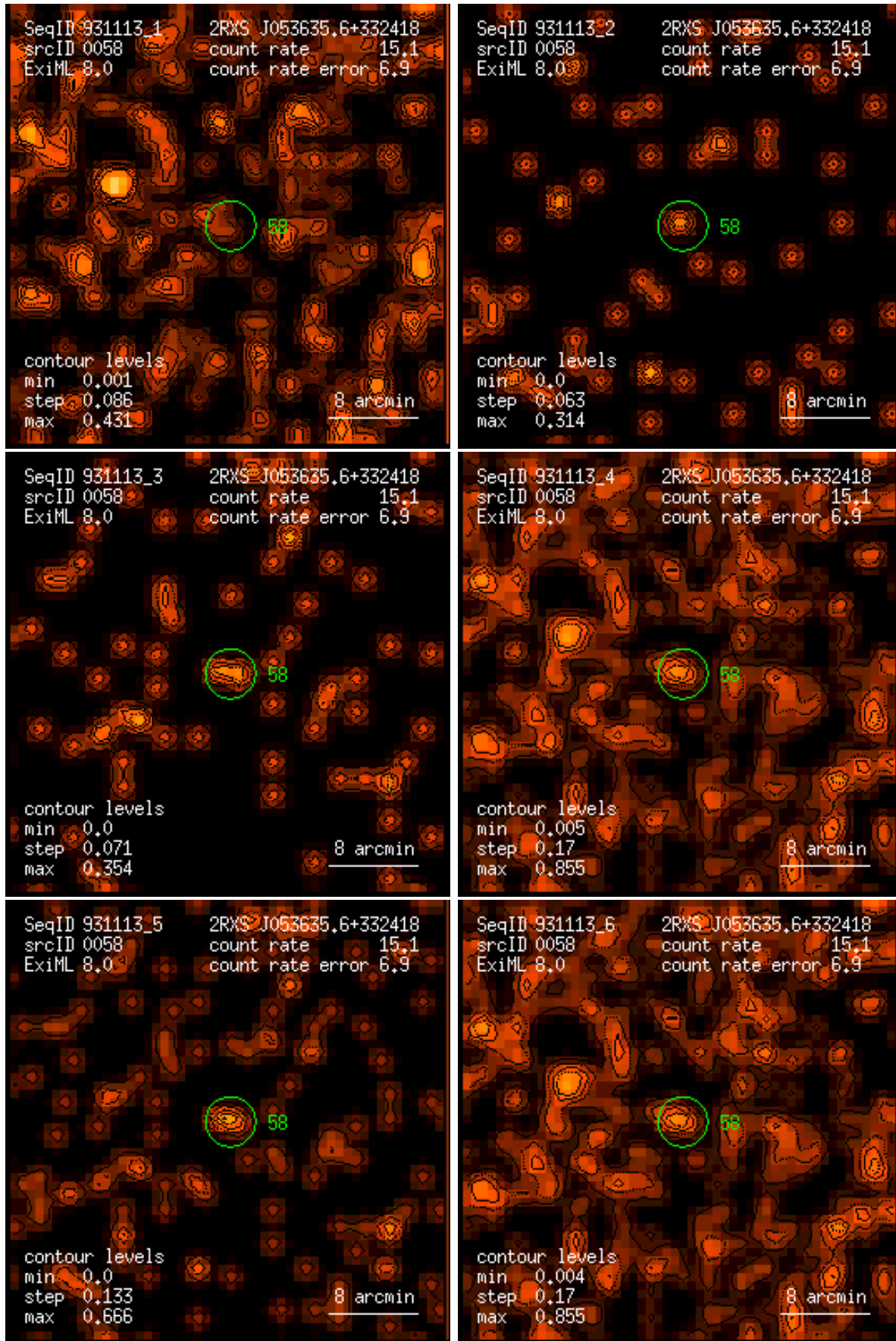
Figure 58: RASS 931113: detection 0058: band rate images, Gaussian filter: (1) PSPC channels 11 – 41, (2) 52 – 90, (3) 91 – 201, (4) 11 – 235, (5) 52 – 201, (6) 11 – 201. Broad band rates in counts/ks. Band rate contour levels in counts/ks/arcmin 2 .
