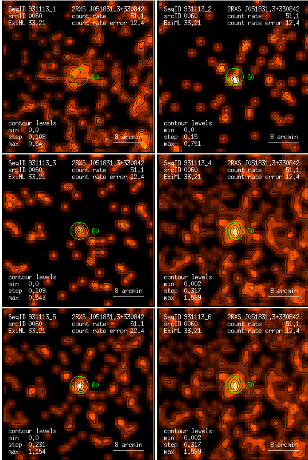
Figure 60: RASS 931113: detection 0060: band rate images, Gaussian filter: (1) PSPC channels 11 – 41, (2) 52 – 90, (3) 91 – 201, (4) 11 – 235, (5) 52 – 201, (6) 11 – 201. Broad band rates in counts/ks. Band rate contour levels in counts/ks/arcmin 2 .
