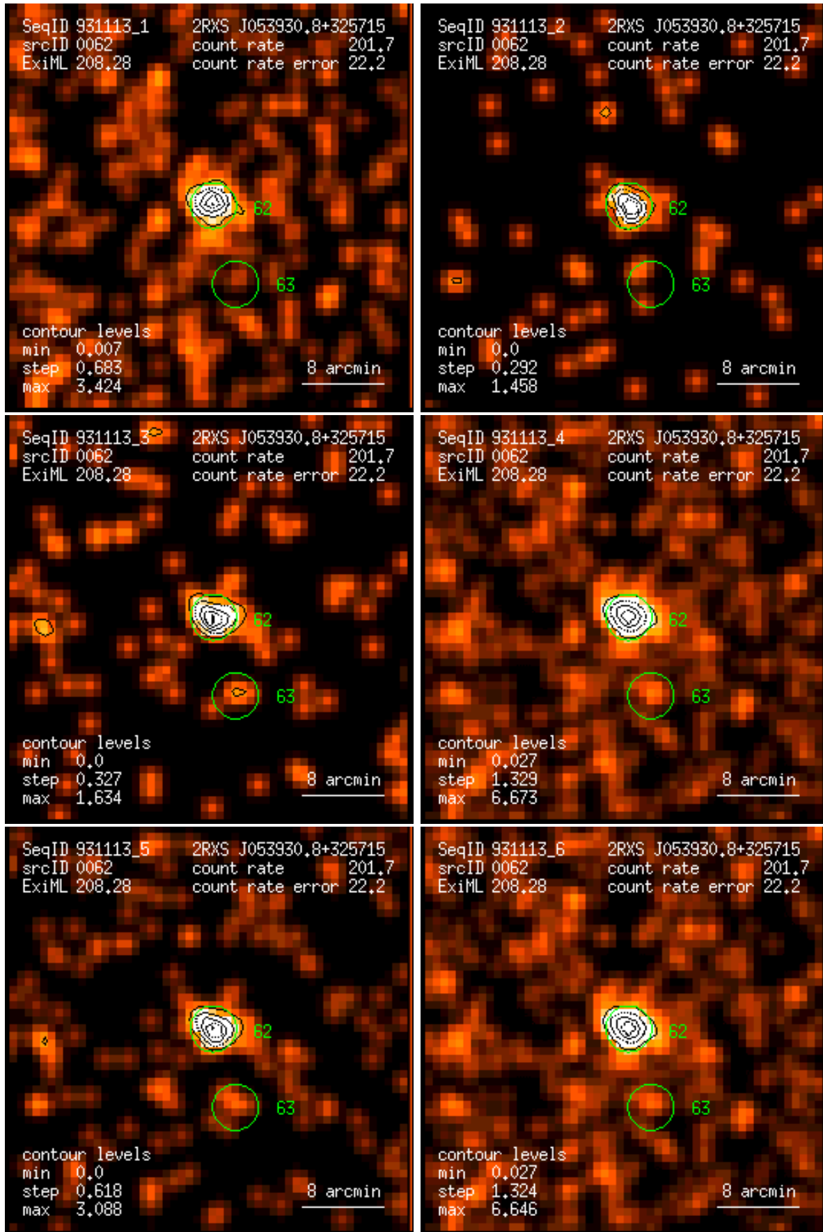
Figure 62: RASS 931113: detection 0062: band rate images, Gaussian filter: (1) PSPC channels 11 – 41, (2) 52 – 90, (3) 91 – 201, (4) 11 – 235, (5) 52 – 201, (6) 11 – 201. Broad band rates in counts/ks. Band rate contour levels in counts/ks/arcmin 2 .
