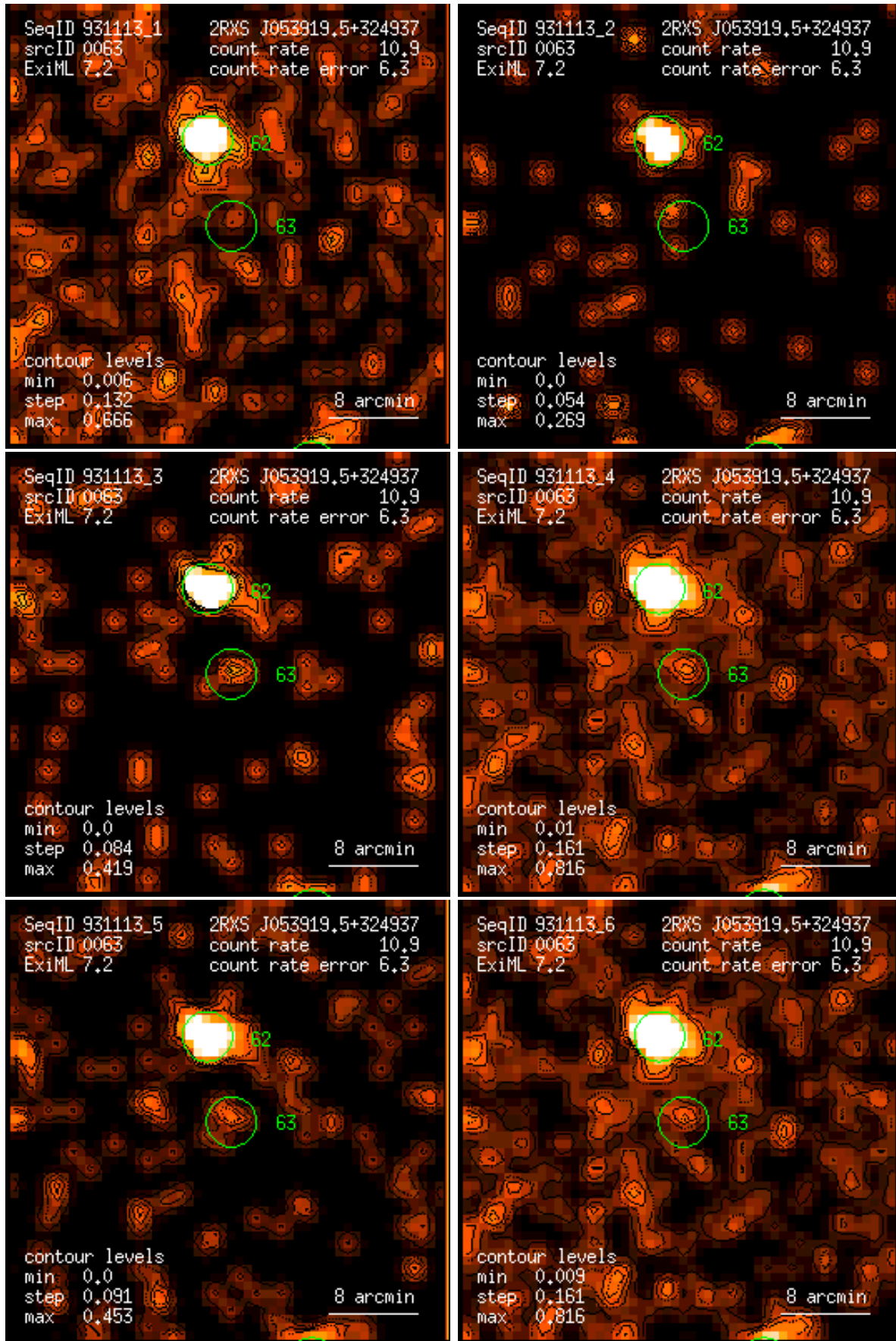
Figure 63: RASS 931113: detection 0063: band rate images, Gaussian filter: (1) PSPC channels 11 – 41, (2) 52 – 90, (3) 91 – 201, (4) 11 – 235, (5) 52 – 201, (6) 11 – 201. Broad band rates in counts/ks. Band rate contour levels in counts/ks/arcmin 2 .
