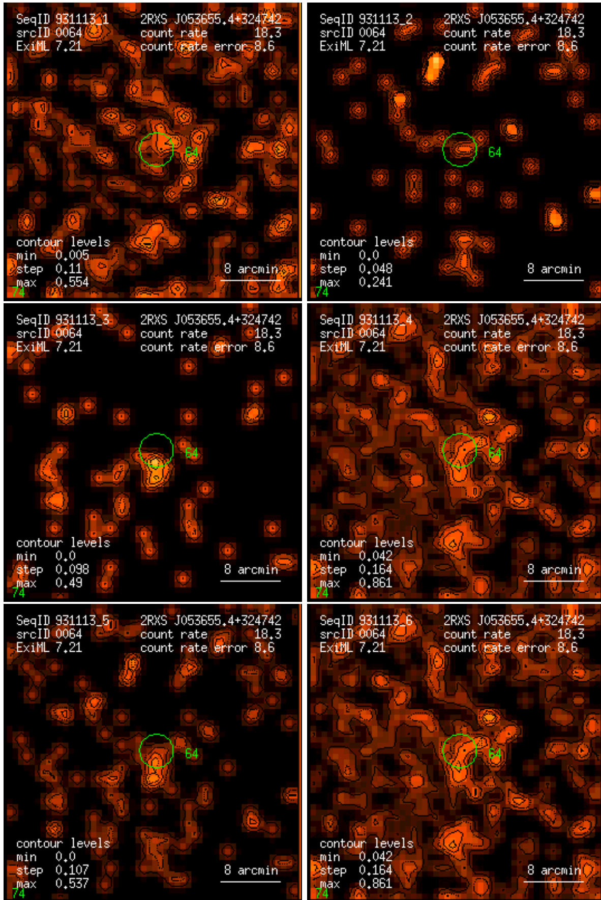
Figure 64: RASS 931113: detection 0064: band rate images, Gaussian filter: (1) PSPC channels 11 – 41, (2) 52 – 90, (3) 91 – 201, (4) 11 – 235, (5) 52 – 201, (6) 11 – 201. Broad band rates in counts/ks. Band rate contour levels in counts/ks/arcmin 2 .
