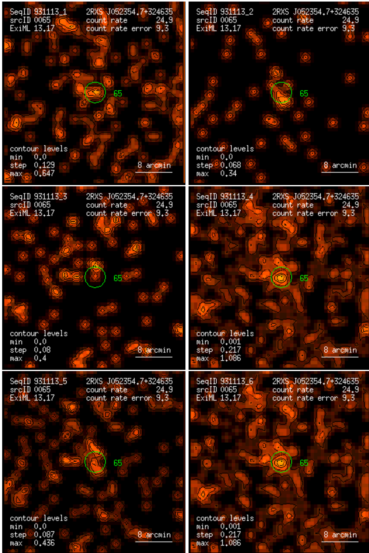
Figure 65: RASS 931113: detection 0065: band rate images, Gaussian filter: (1) PSPC channels 11 – 41, (2) 52 – 90, (3) 91 – 201, (4) 11 – 235, (5) 52 – 201, (6) 11 – 201. Broad band rates in counts/ks. Band rate contour levels in counts/ks/arcmin 2 .
