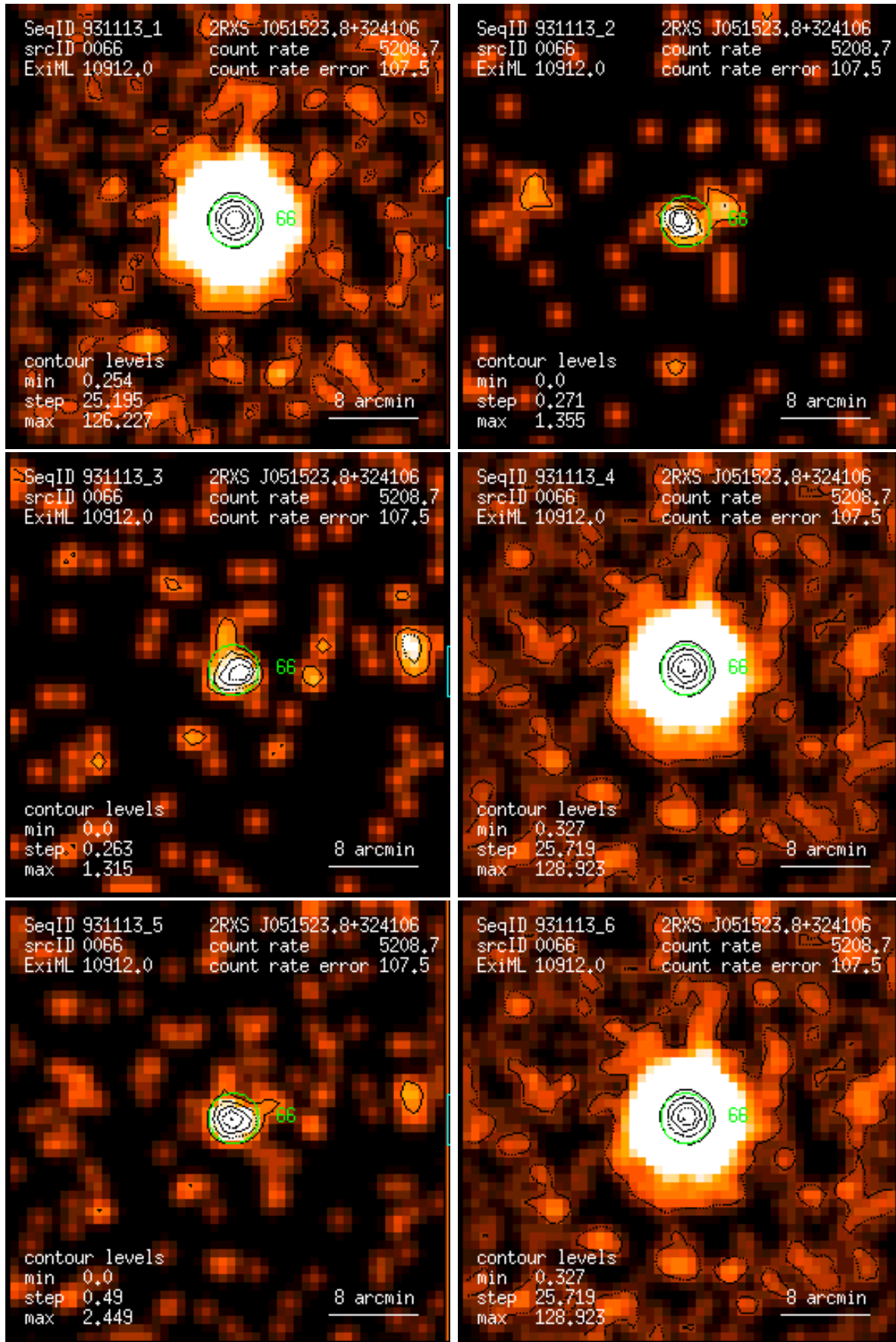
Figure 66: RASS 931113: detection 0066: band rate images, Gaussian filter: (1) PSPC channels 11 – 41, (2) 52 – 90, (3) 91 – 201, (4) 11 – 235, (5) 52 – 201, (6) 11 – 201. Broad band rates in counts/ks. Band rate contour levels in counts/ks/arcmin 2 .
