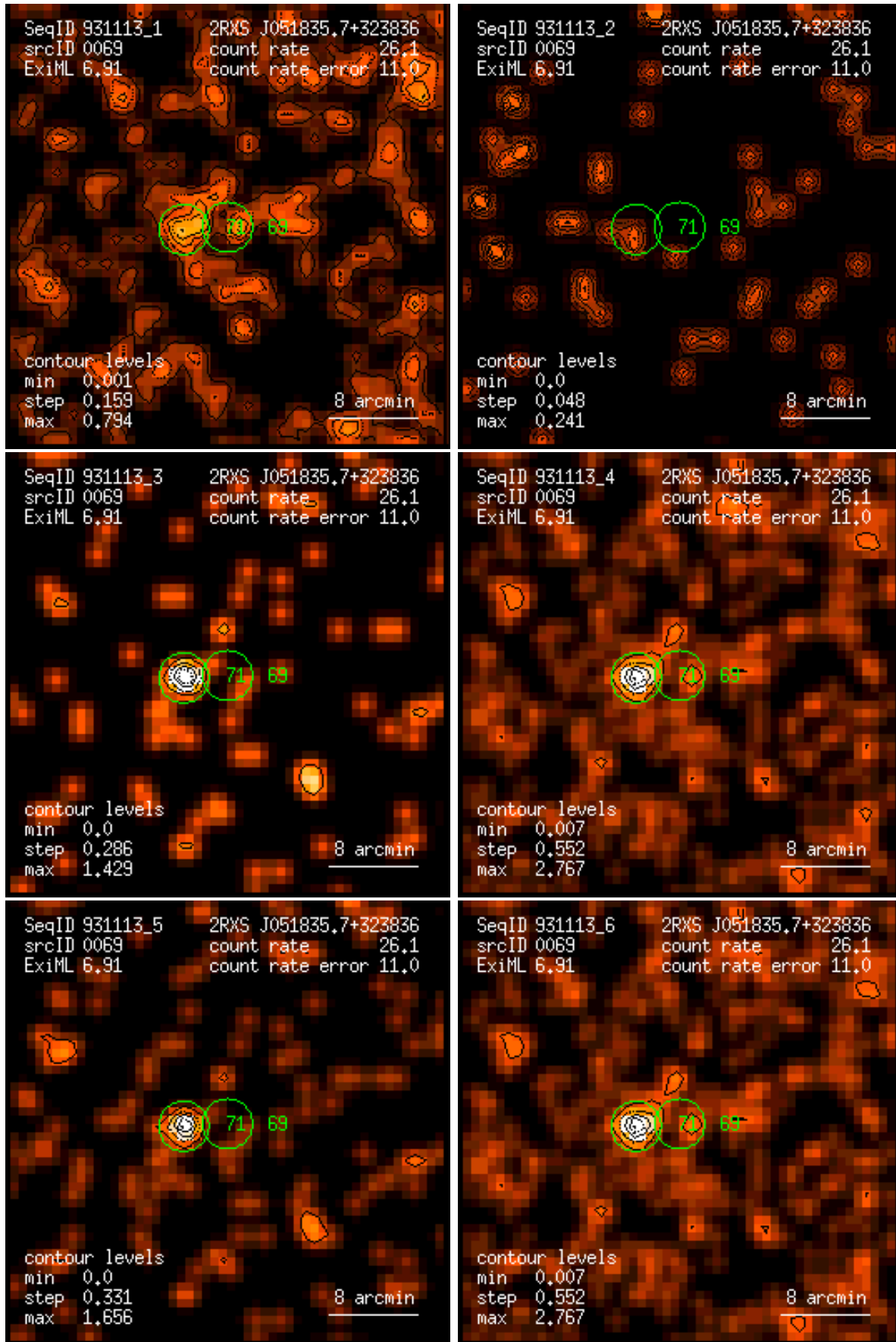
Figure 69: RASS 931113: detection 0069: band rate images, Gaussian filter: (1) PSPC channels 11 – 41, (2) 52 – 90, (3) 91 – 201, (4) 11 – 235, (5) 52 – 201, (6) 11 – 201. Broad band rates in counts/ks. Band rate contour levels in counts/ks/arcmin 2 .
