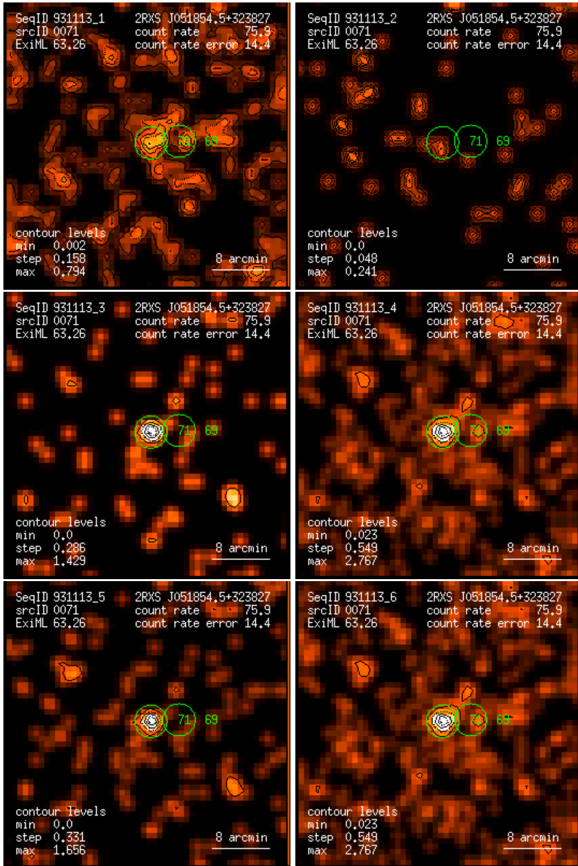
Figure 71: RASS 931113: detection 0071: band rate images, Gaussian filter: (1) PSPC channels 11 – 41, (2) 52 – 90, (3) 91 – 201, (4) 11 – 235, (5) 52 – 201, (6) 11 – 201. Broad band rates in counts/ks. Band rate contour levels in counts/ks/arcmin 2 .
