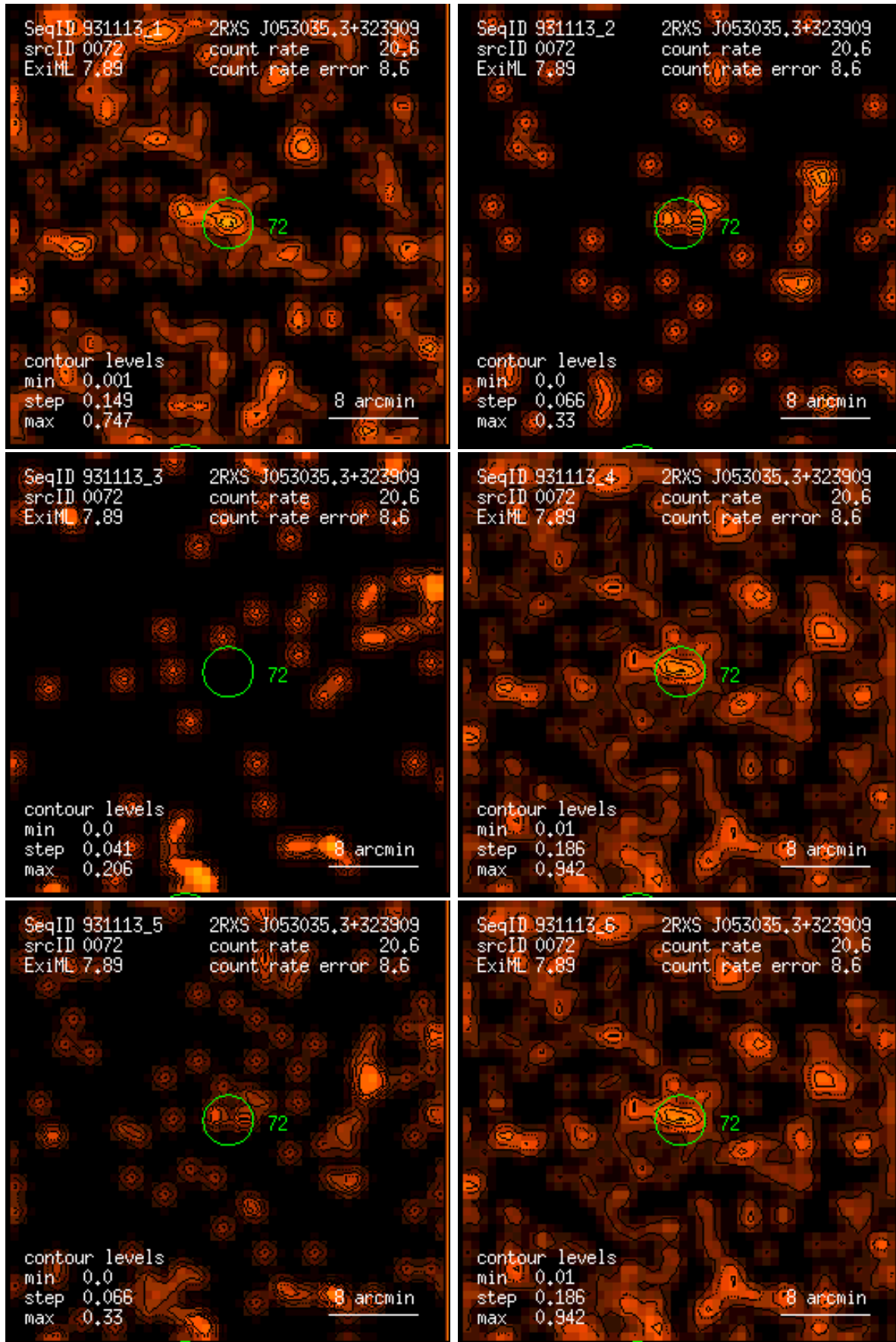
Figure 72: RASS 931113: detection 0072: band rate images, Gaussian filter: (1) PSPC channels 11 – 41, (2) 52 – 90, (3) 91 – 201, (4) 11 – 235, (5) 52 – 201, (6) 11 – 201. Broad band rates in counts/ks. Band rate contour levels in counts/ks/arcmin 2 .
