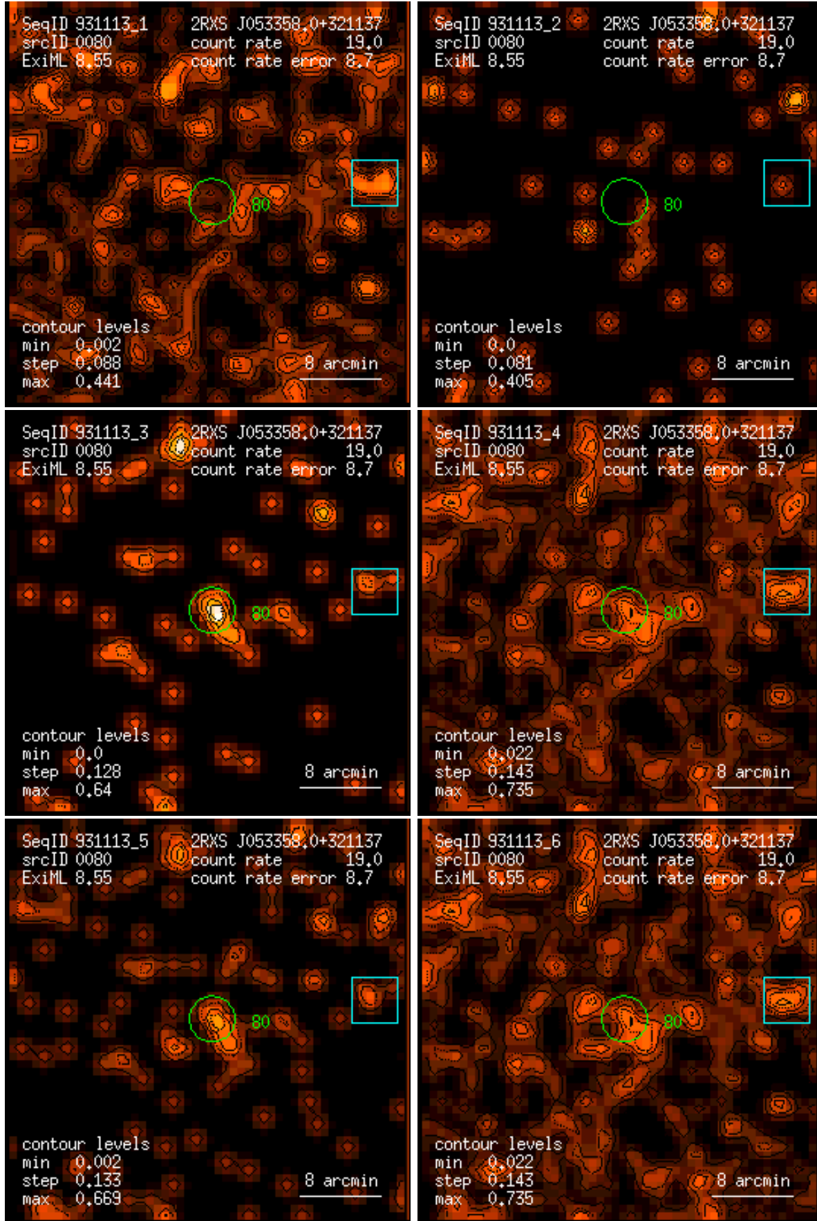
Figure 80: RASS 931113: detection 0080: band rate images, Gaussian filter: (1) PSPC channels 11 – 41, (2) 52 – 90, (3) 91 – 201, (4) 11 – 235, (5) 52 – 201, (6) 11 – 201. Broad band rates in counts/ks. Band rate contour levels in counts/ks/arcmin 2 .
