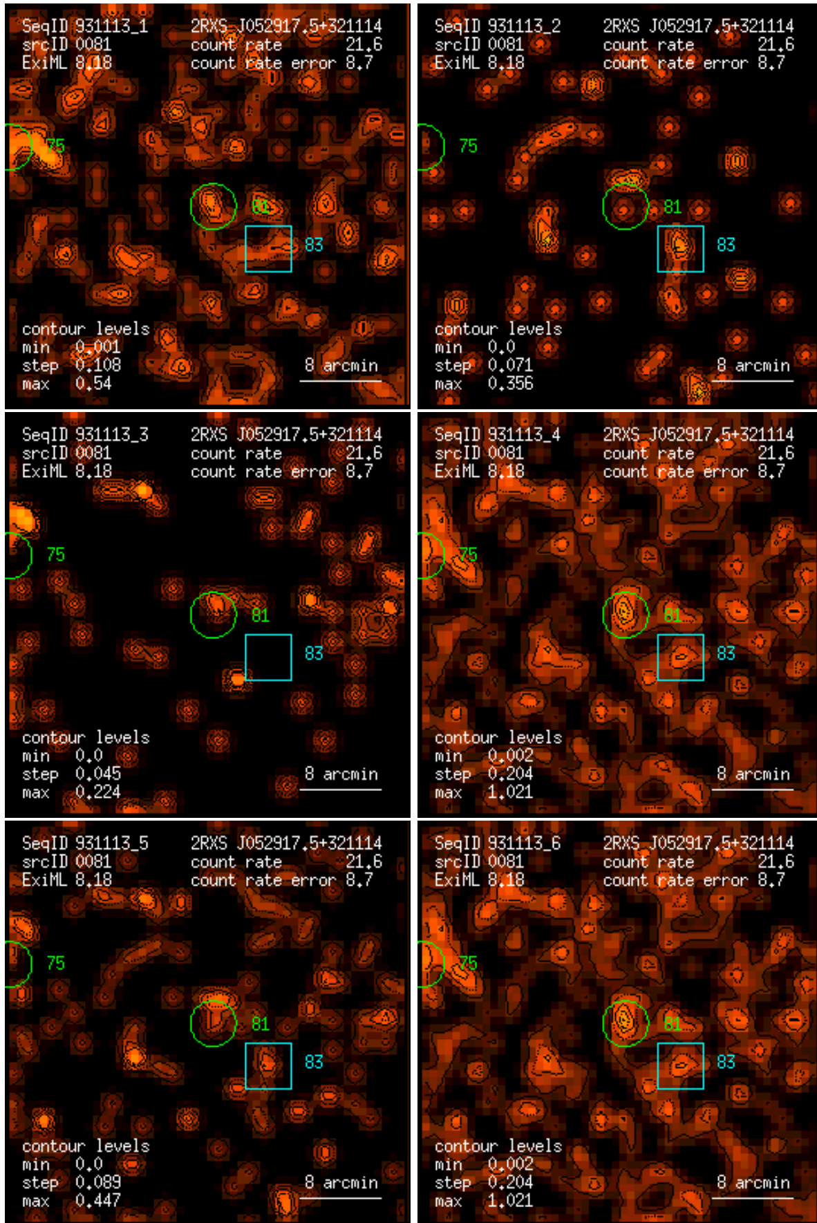
Figure 81: RASS 931113: detection 0081: band rate images, Gaussian filter: (1) PSPC channels 11 – 41, (2) 52 – 90, (3) 91 – 201, (4) 11 – 235, (5) 52 – 201, (6) 11 – 201. Broad band rates in counts/ks. Band rate contour levels in counts/ks/arcmin 2 .
