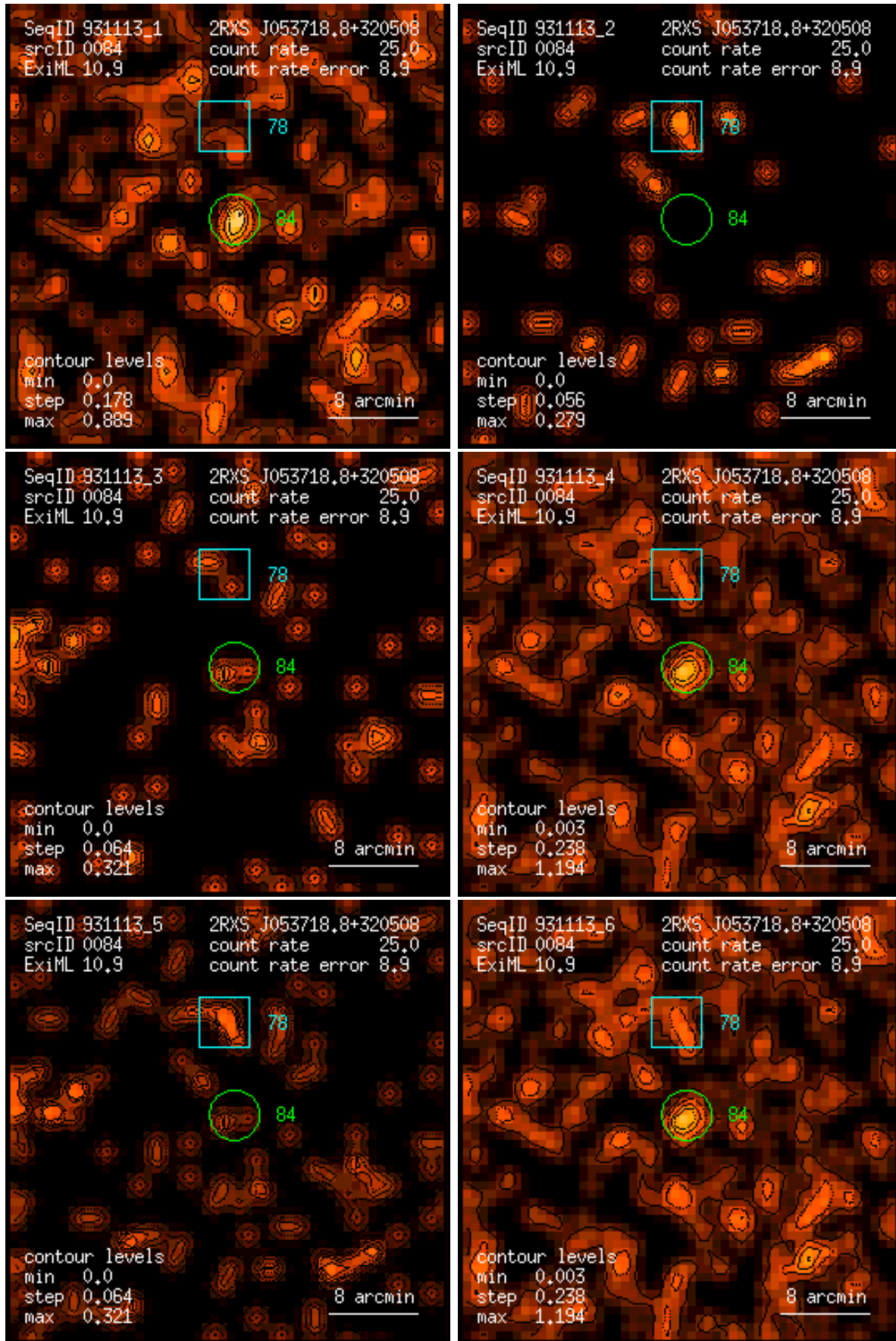
Figure 84: RASS 931113: detection 0084: band rate images, Gaussian filter: (1) PSPC channels 11 – 41, (2) 52 – 90, (3) 91 – 201, (4) 11 – 235, (5) 52 – 201, (6) 11 – 201. Broad band rates in counts/ks. Band rate contour levels in counts/ks/arcmin 2 .
