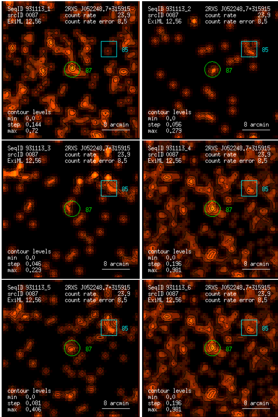
Figure 87: RASS 931113: detection 0087: band rate images, Gaussian filter: (1) PSPC channels 11 – 41, (2) 52 – 90, (3) 91 – 201, (4) 11 – 235, (5) 52 – 201, (6) 11 – 201. Broad band rates in counts/ks. Band rate contour levels in counts/ks/arcmin 2 .
