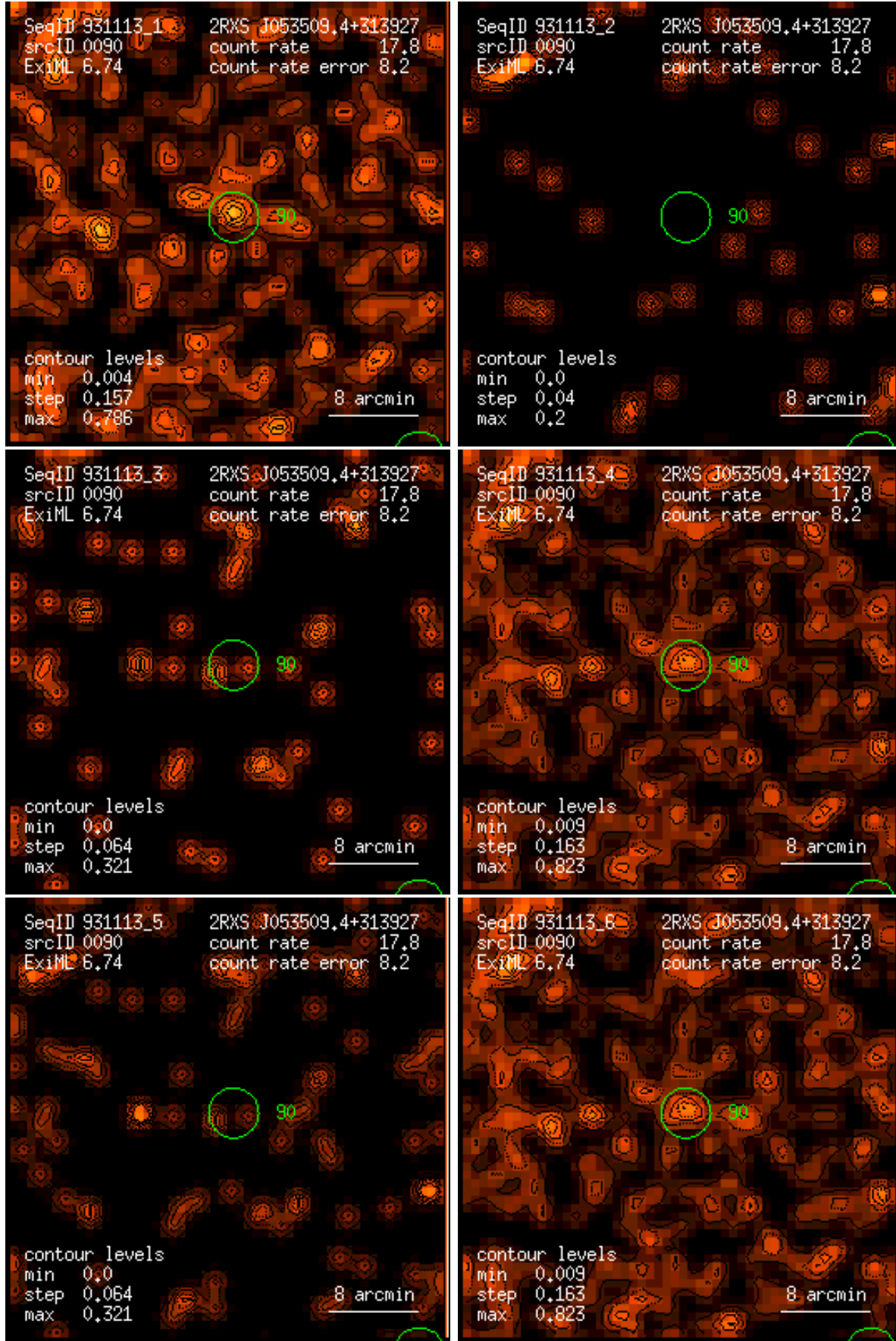
Figure 90: RASS 931113: detection 0090: band rate images, Gaussian filter: (1) PSPC channels 11 – 41, (2) 52 – 90, (3) 91 – 201, (4) 11 – 235, (5) 52 – 201, (6) 11 – 201. Broad band rates in counts/ks. Band rate contour levels in counts/ks/arcmin 2 .
