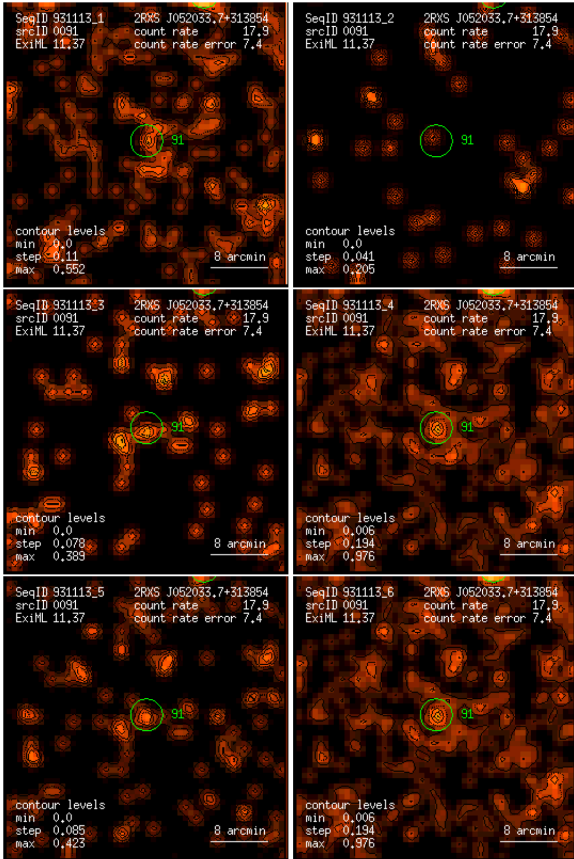
Figure 91: RASS 931113: detection 0091: band rate images, Gaussian filter: (1) PSPC channels 11 – 41, (2) 52 – 90, (3) 91 – 201, (4) 11 – 235, (5) 52 – 201, (6) 11 – 201. Broad band rates in counts/ks. Band rate contour levels in counts/ks/arcmin 2 .
