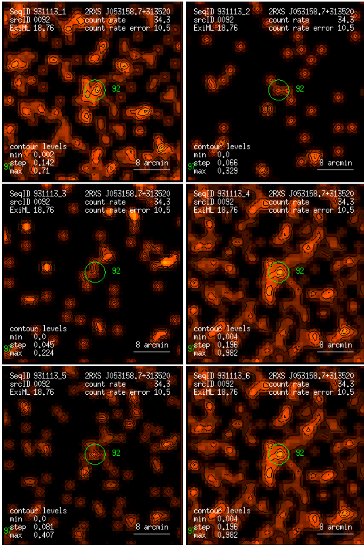
Figure 92: RASS 931113: detection 0092: band rate images, Gaussian filter: (1) PSPC channels 11 – 41, (2) 52 – 90, (3) 91 – 201, (4) 11 – 235, (5) 52 – 201, (6) 11 – 201. Broad band rates in counts/ks. Band rate contour levels in counts/ks/arcmin 2 .
