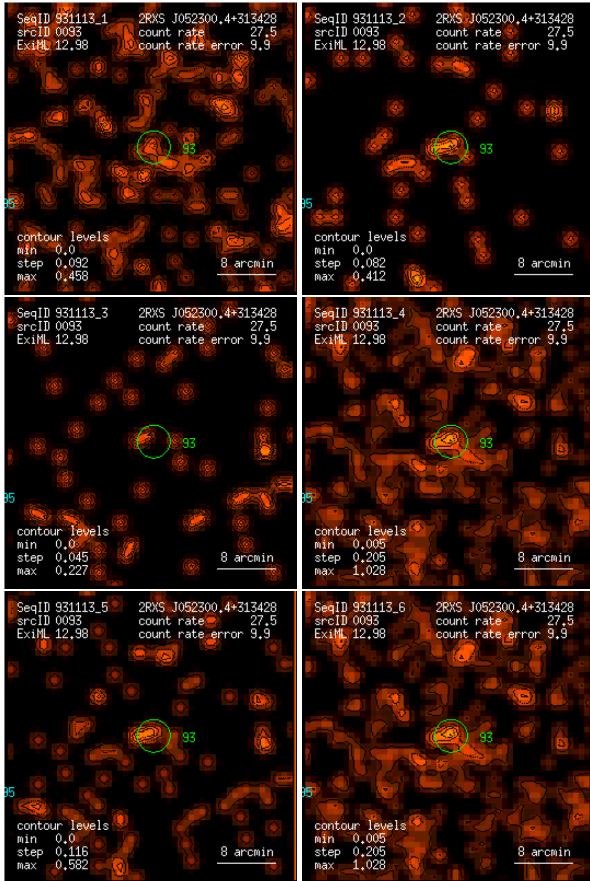
Figure 93: RASS 931113: detection 0093: band rate images, Gaussian filter: (1) PSPC channels 11 – 41, (2) 52 – 90, (3) 91 – 201, (4) 11 – 235, (5) 52 – 201, (6) 11 – 201. Broad band rates in counts/ks. Band rate contour levels in counts/ks/arcmin 2 .
