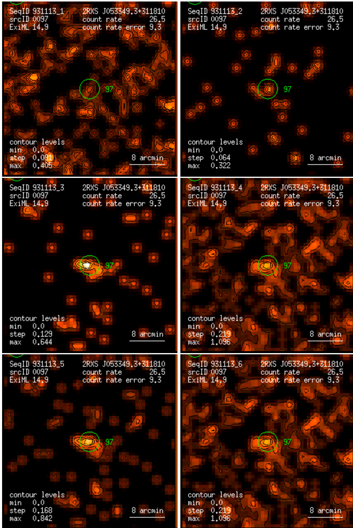
Figure 97: RASS 931113: detection 0097: band rate images, Gaussian filter: (1) PSPC channels 11 – 41, (2) 52 – 90, (3) 91 – 201, (4) 11 – 235, (5) 52 – 201, (6) 11 – 201. Broad band rates in counts/ks. Band rate contour levels in counts/ks/arcmin 2 .
