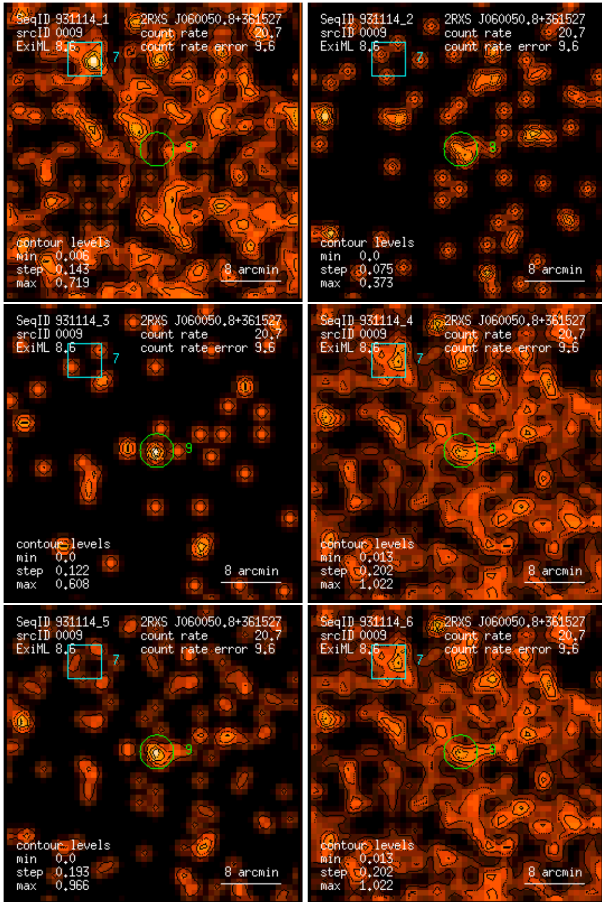
Figure 9: RASS 931114: detection 0009: band rate images, Gaussian filter: (1) PSPC channels 11 – 41, (2) 52 – 90, (3) 91 – 201, (4) 11 – 235, (5) 52 – 201, (6) 11 – 201. Broad band rates in counts/ks. Band rate contour levels in counts/ks/arcmin 2 .
