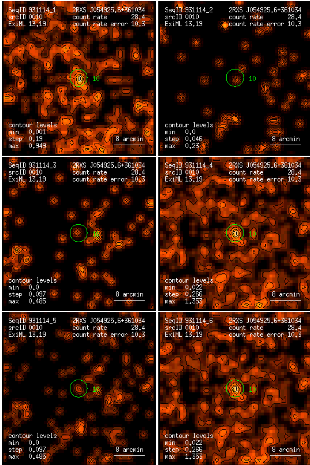
Figure 10: RASS 931114: detection 0010: band rate images, Gaussian filter: (1) PSPC channels 11 – 41, (2) 52 – 90, (3) 91 – 201, (4) 11 – 235, (5) 52 – 201, (6) 11 – 201. Broad band rates in counts/ks. Band rate contour levels in counts/ks/arcmin 2 .
