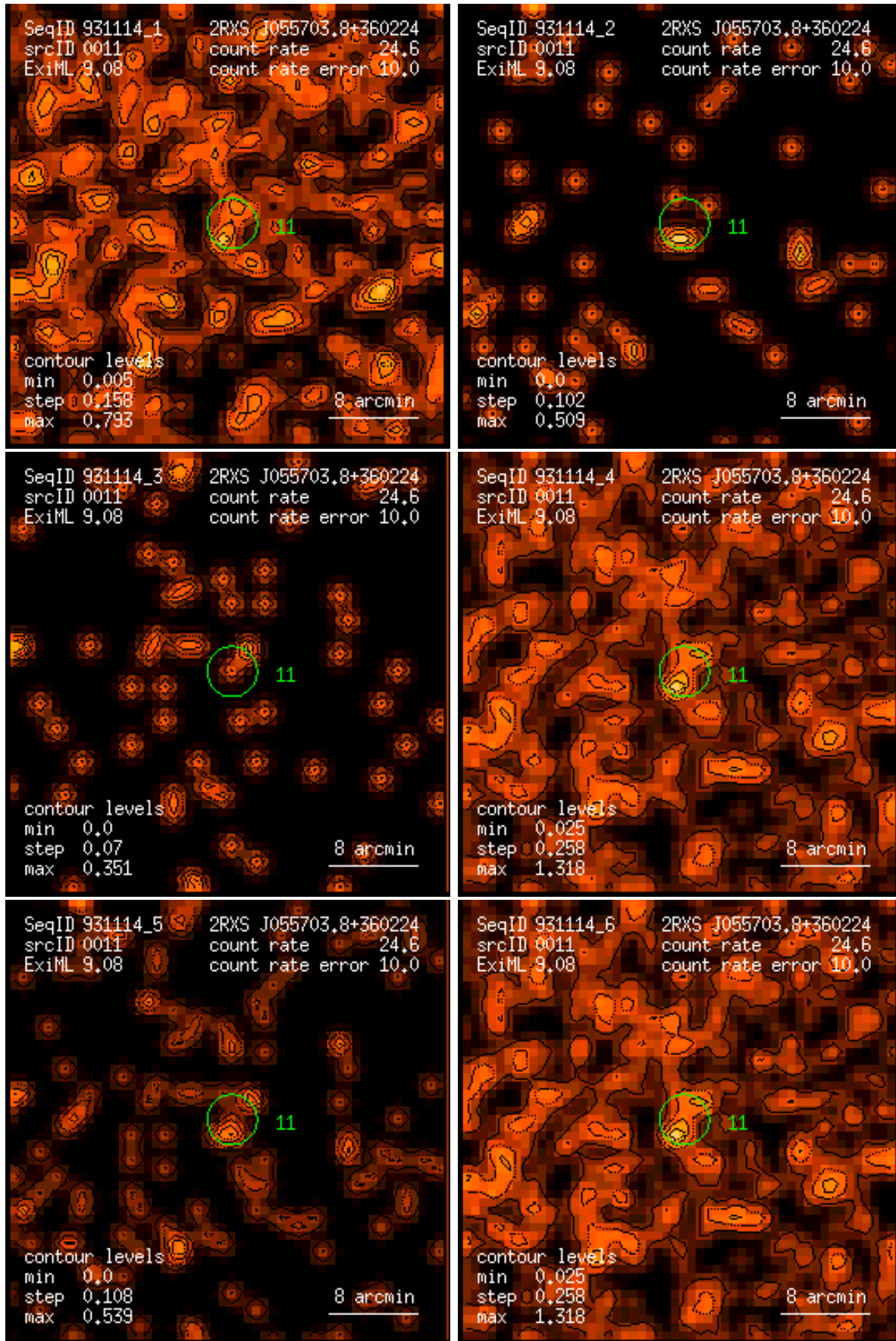
Figure 11: RASS 931114: detection 0011: band rate images, Gaussian filter: (1) PSPC channels 11 – 41, (2) 52 – 90, (3) 91 – 201, (4) 11 – 235, (5) 52 – 201, (6) 11 – 201. Broad band rates in counts/ks. Band rate contour levels in counts/ks/arcmin 2 .
