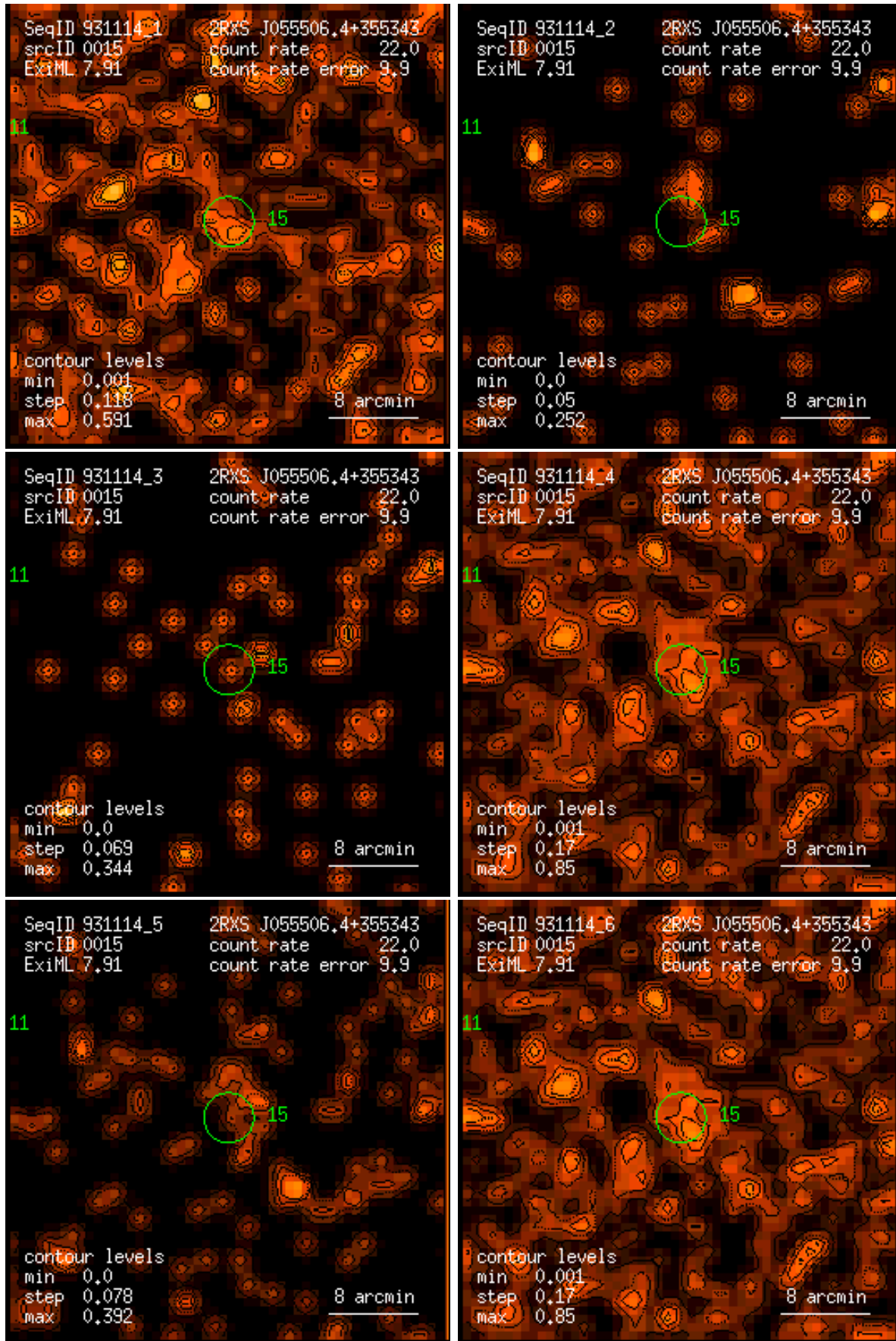
Figure 15: RASS 931114: detection 0015: band rate images, Gaussian filter: (1) PSPC channels 11 – 41, (2) 52 – 90, (3) 91 – 201, (4) 11 – 235, (5) 52 – 201, (6) 11 – 201. Broad band rates in counts/ks. Band rate contour levels in counts/ks/arcmin 2 .
