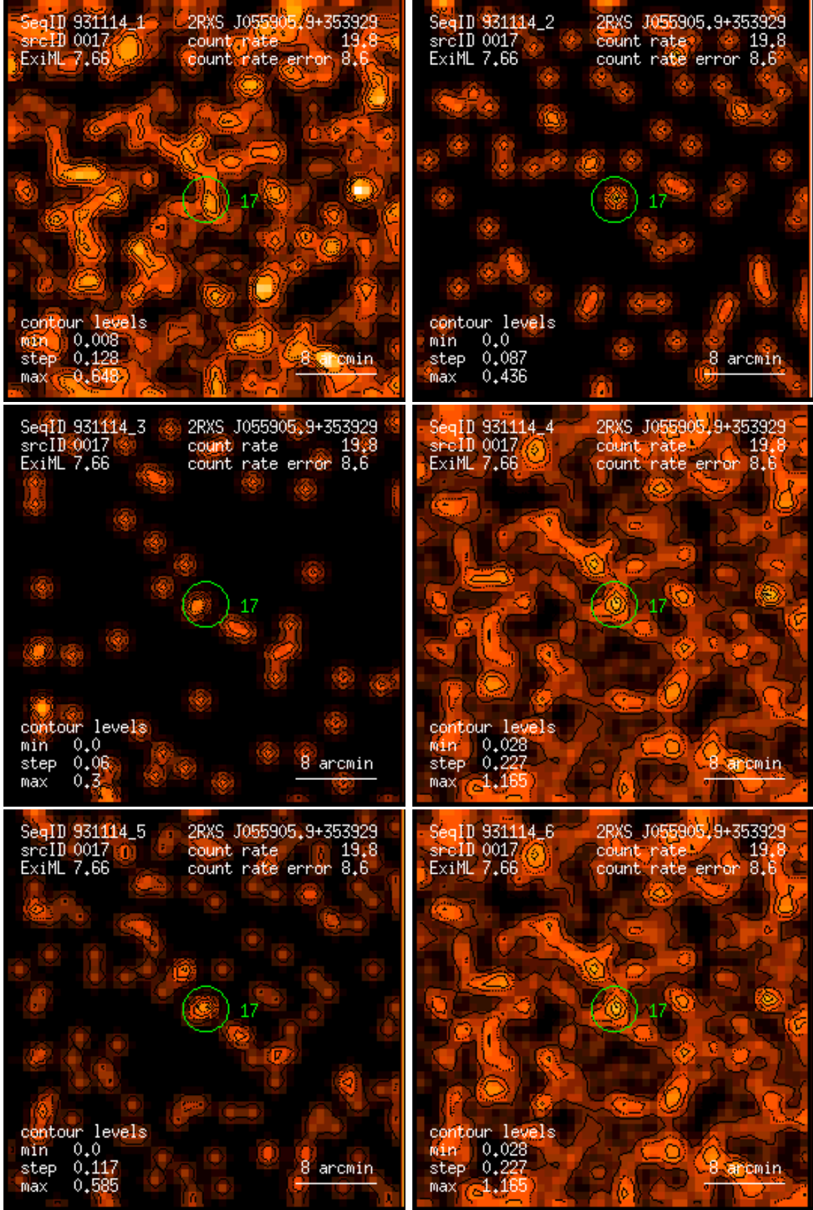
Figure 17: RASS 931114: detection 0017: band rate images, Gaussian filter: (1) PSPC channels 11 – 41, (2) 52 – 90, (3) 91 – 201, (4) 11 – 235, (5) 52 – 201, (6) 11 – 201. Broad band rates in counts/ks. Band rate contour levels in counts/ks/arcmin 2 .
