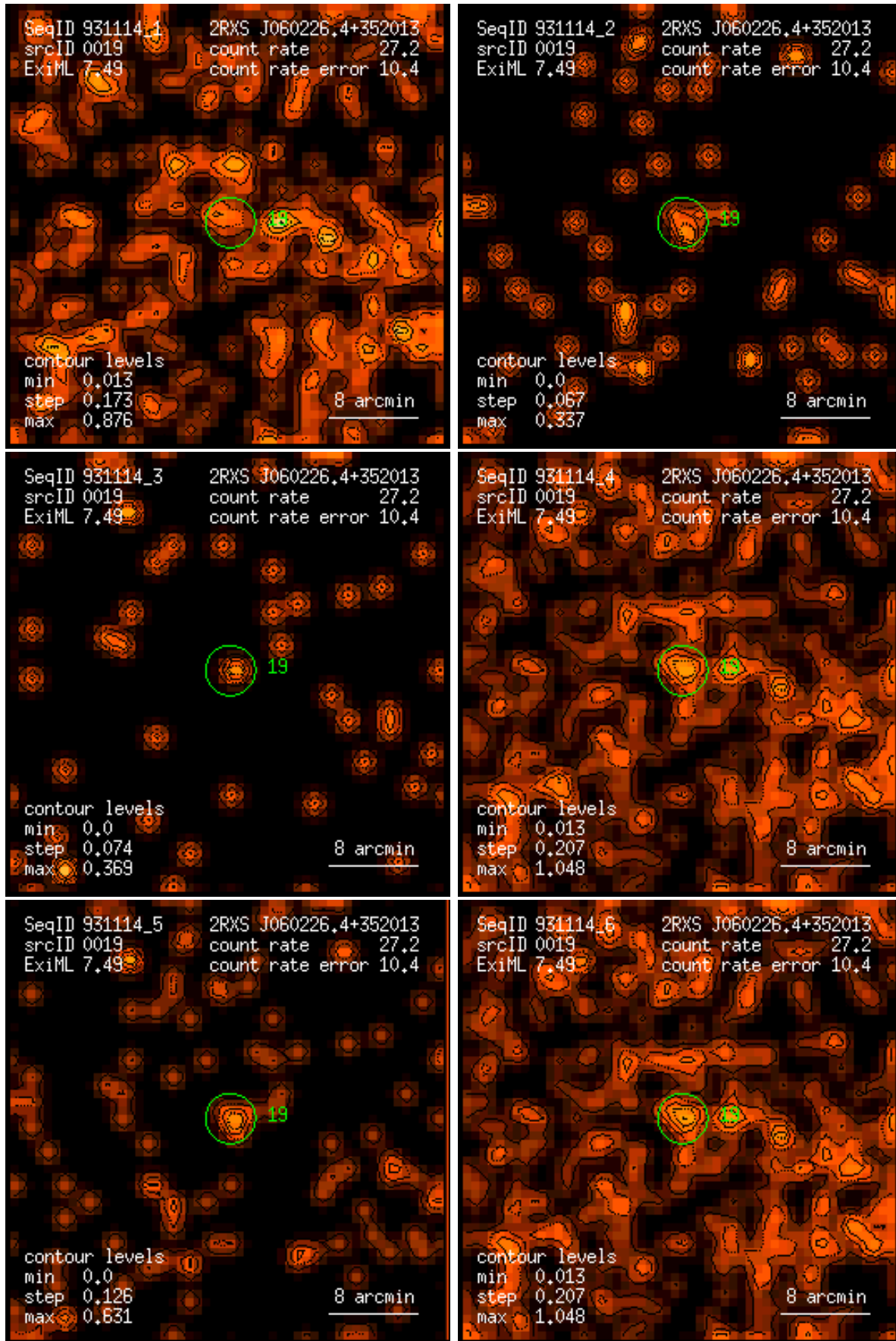
Figure 19: RASS 931114: detection 0019: band rate images, Gaussian filter: (1) PSPC channels 11 – 41, (2) 52 – 90, (3) 91 – 201, (4) 11 – 235, (5) 52 – 201, (6) 11 – 201. Broad band rates in counts/ks. Band rate contour levels in counts/ks/arcmin 2 .
