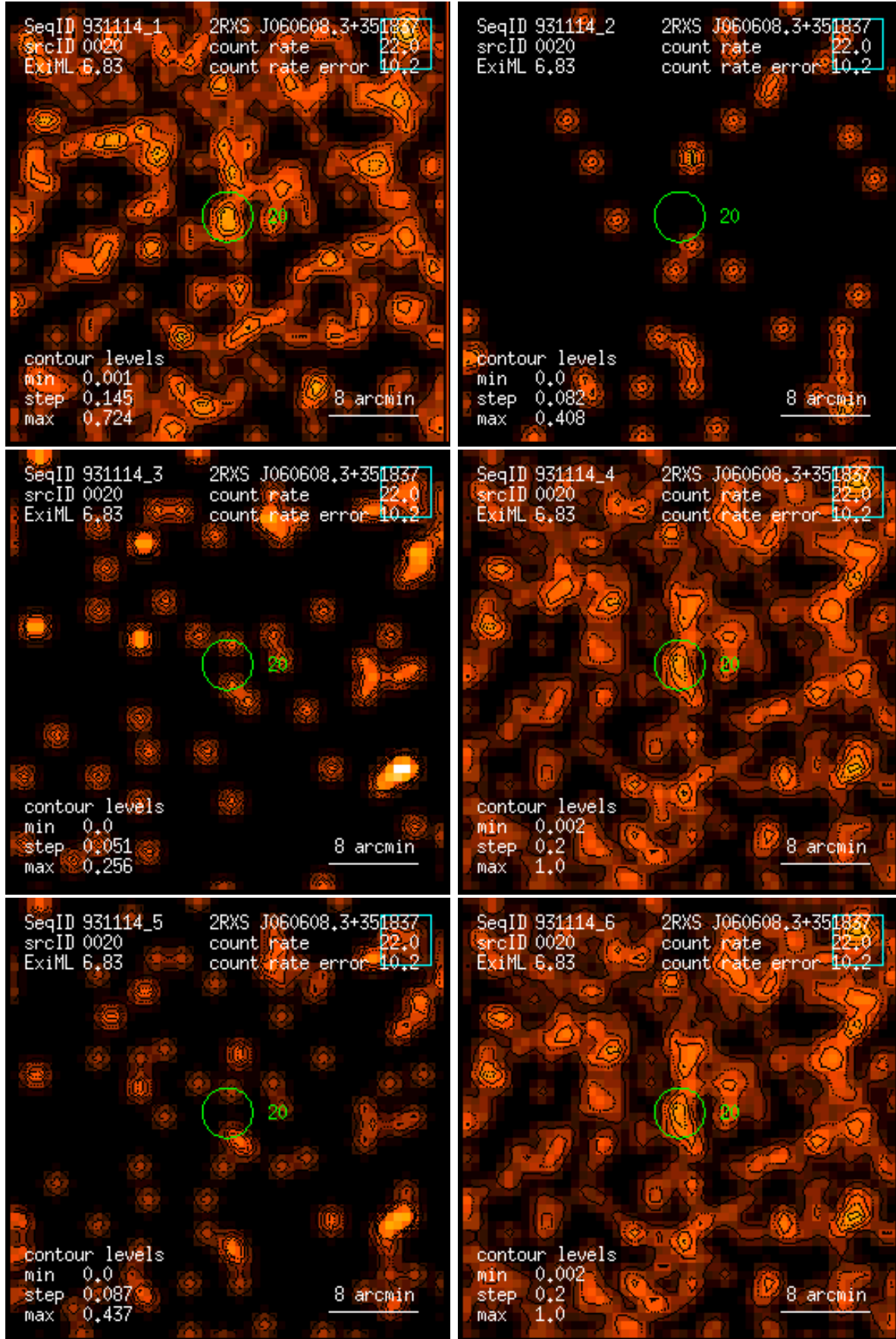
Figure 20: RASS 931114: detection 0020: band rate images, Gaussian filter: (1) PSPC channels 11 – 41, (2) 52 – 90, (3) 91 – 201, (4) 11 – 235, (5) 52 – 201, (6) 11 – 201. Broad band rates in counts/ks. Band rate contour levels in counts/ks/arcmin 2 .
