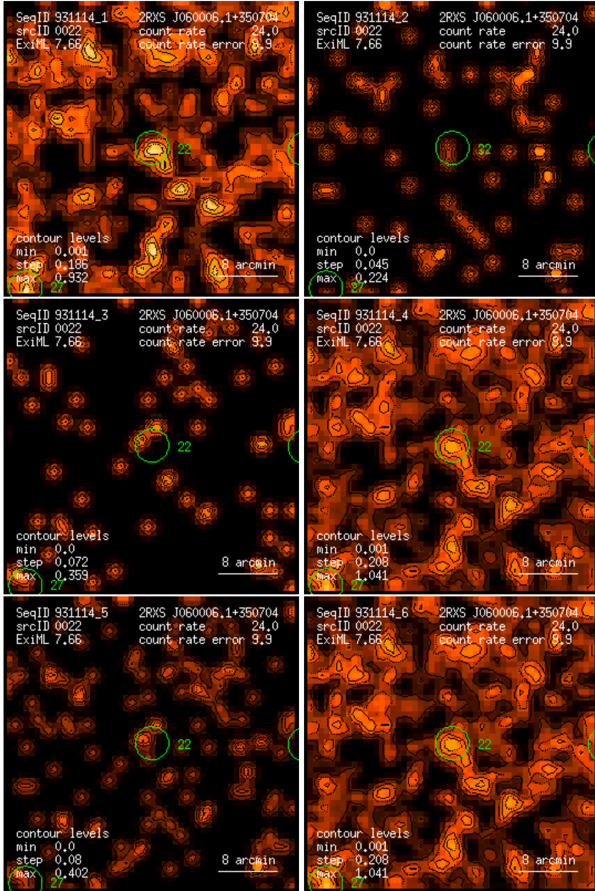
Figure 22: RASS 931114: detection 0022: band rate images, Gaussian filter: (1) PSPC channels 11 – 41, (2) 52 – 90, (3) 91 – 201, (4) 11 – 235, (5) 52 – 201, (6) 11 – 201. Broad band rates in counts/ks. Band rate contour levels in counts/ks/arcmin 2 .
