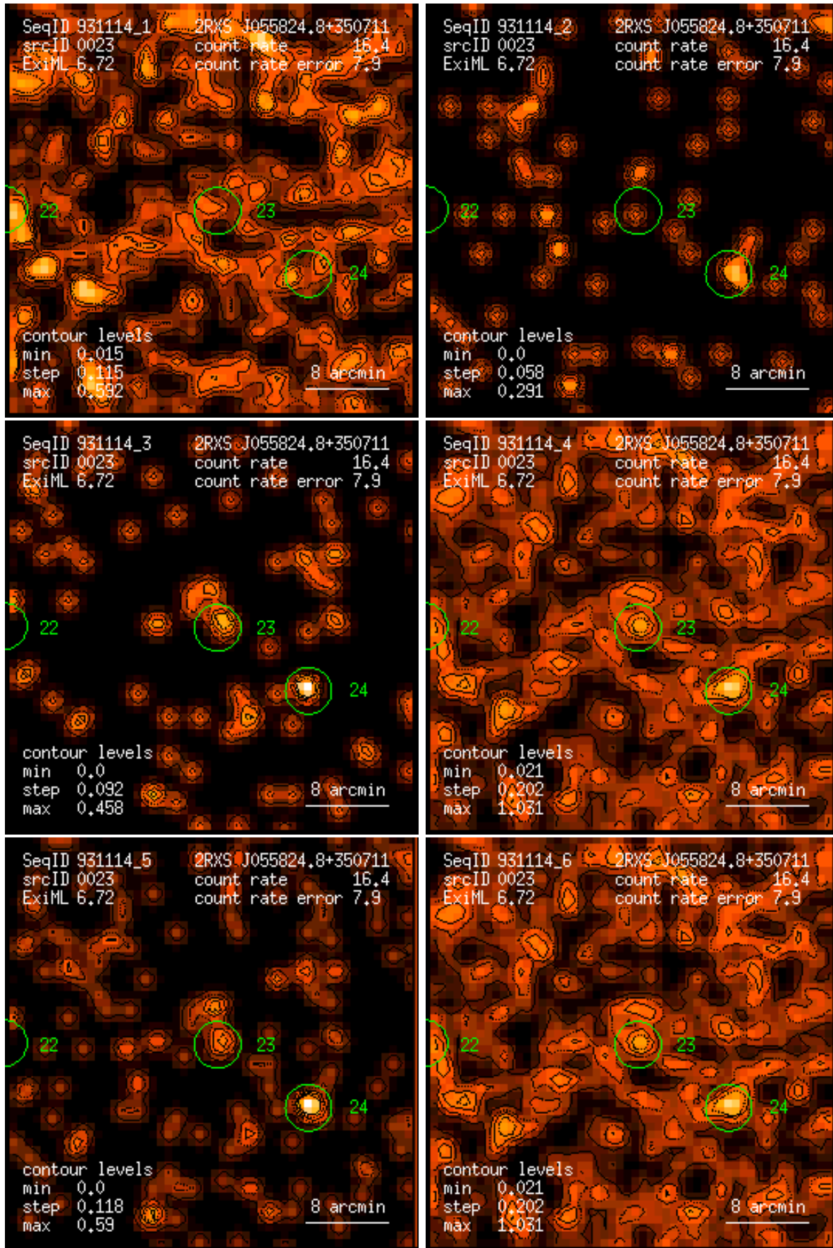
Figure 23: RASS 931114: detection 0023: band rate images, Gaussian filter: (1) PSPC channels 11 – 41, (2) 52 – 90, (3) 91 – 201, (4) 11 – 235, (5) 52 – 201, (6) 11 – 201. Broad band rates in counts/ks. Band rate contour levels in counts/ks/arcmin 2 .
