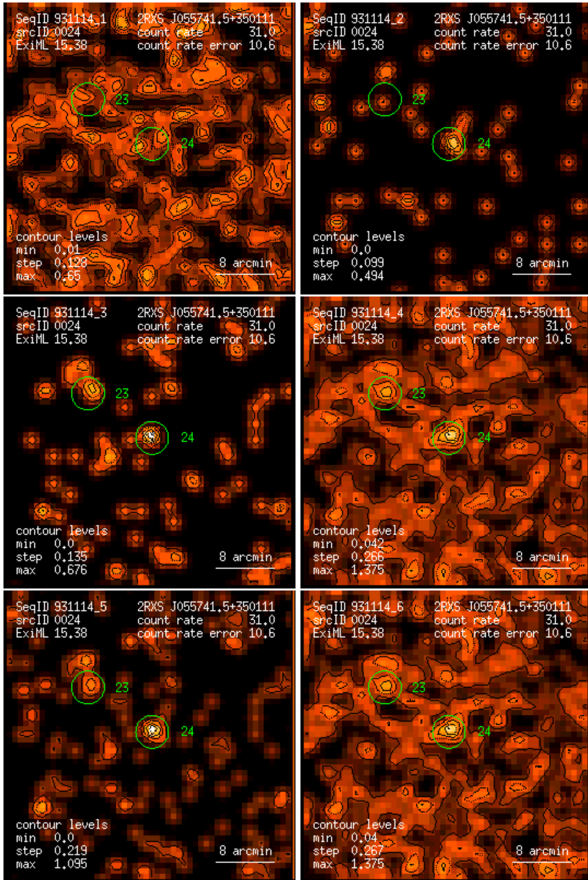
Figure 24: RASS 931114: detection 0024: band rate images, Gaussian filter: (1) PSPC channels 11 – 41, (2) 52 – 90, (3) 91 – 201, (4) 11 – 235, (5) 52 – 201, (6) 11 – 201. Broad band rates in counts/ks. Band rate contour levels in counts/ks/arcmin 2 .
