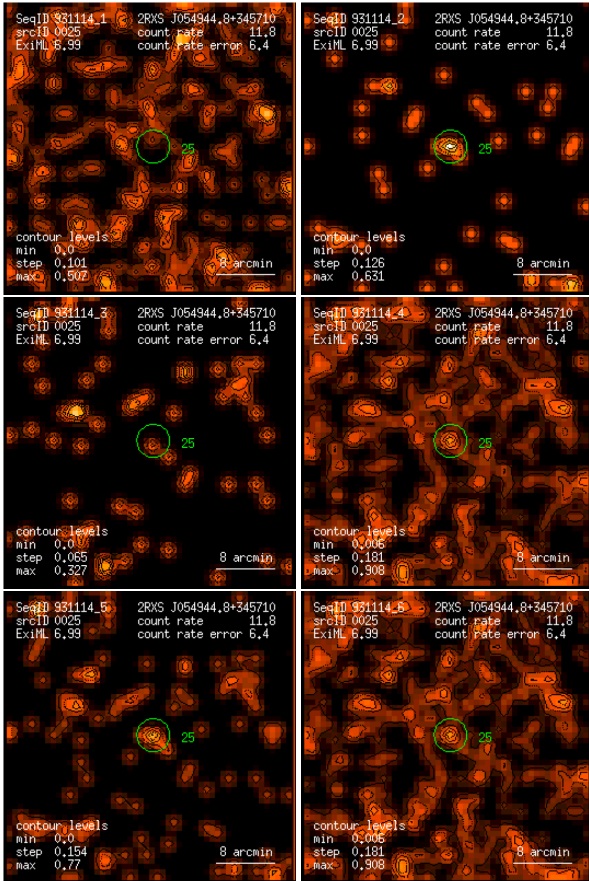
Figure 25: RASS 931114: detection 0025: band rate images, Gaussian filter: (1) PSPC channels 11 – 41, (2) 52 – 90, (3) 91 – 201, (4) 11 – 235, (5) 52 – 201, (6) 11 – 201. Broad band rates in counts/ks. Band rate contour levels in counts/ks/arcmin 2 .
