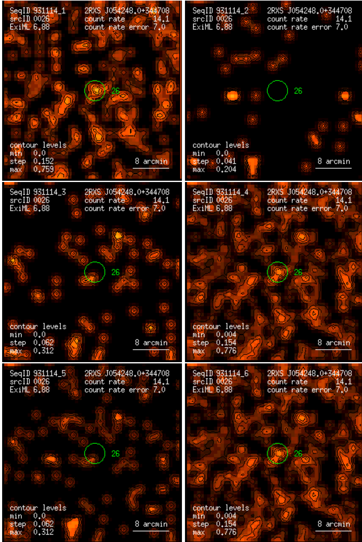
Figure 26: RASS 931114: detection 0026: band rate images, Gaussian filter: (1) PSPC channels 11 – 41, (2) 52 – 90, (3) 91 – 201, (4) 11 – 235, (5) 52 – 201, (6) 11 – 201. Broad band rates in counts/ks. Band rate contour levels in counts/ks/arcmin 2 .
