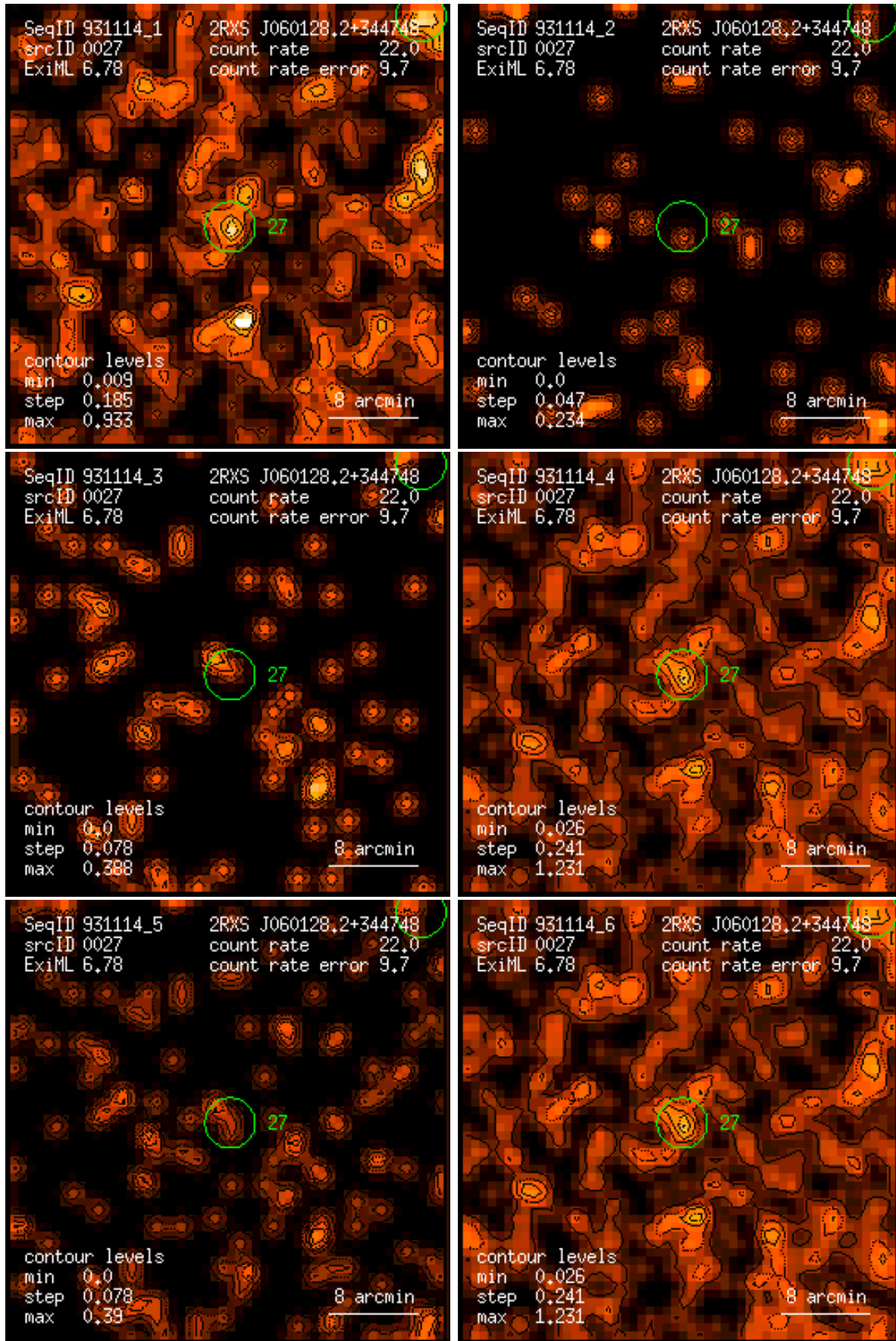
Figure 27: RASS 931114: detection 0027: band rate images, Gaussian filter: (1) PSPC channels 11 – 41, (2) 52 – 90, (3) 91 – 201, (4) 11 – 235, (5) 52 – 201, (6) 11 – 201. Broad band rates in counts/ks. Band rate contour levels in counts/ks/arcmin 2 .
