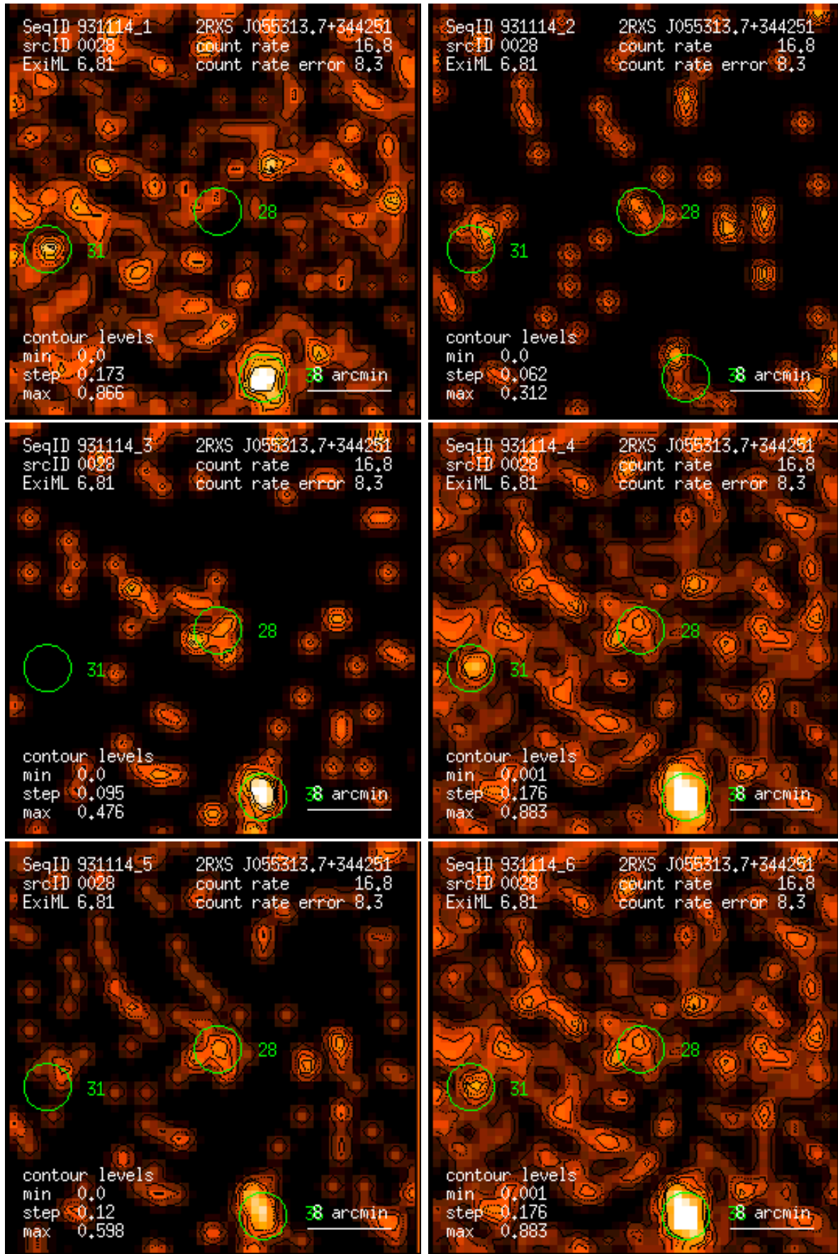
Figure 28: RASS 931114: detection 0028: band rate images, Gaussian filter: (1) PSPC channels 11 – 41, (2) 52 – 90, (3) 91 – 201, (4) 11 – 235, (5) 52 – 201, (6) 11 – 201. Broad band rates in counts/ks. Band rate contour levels in counts/ks/arcmin 2 .
