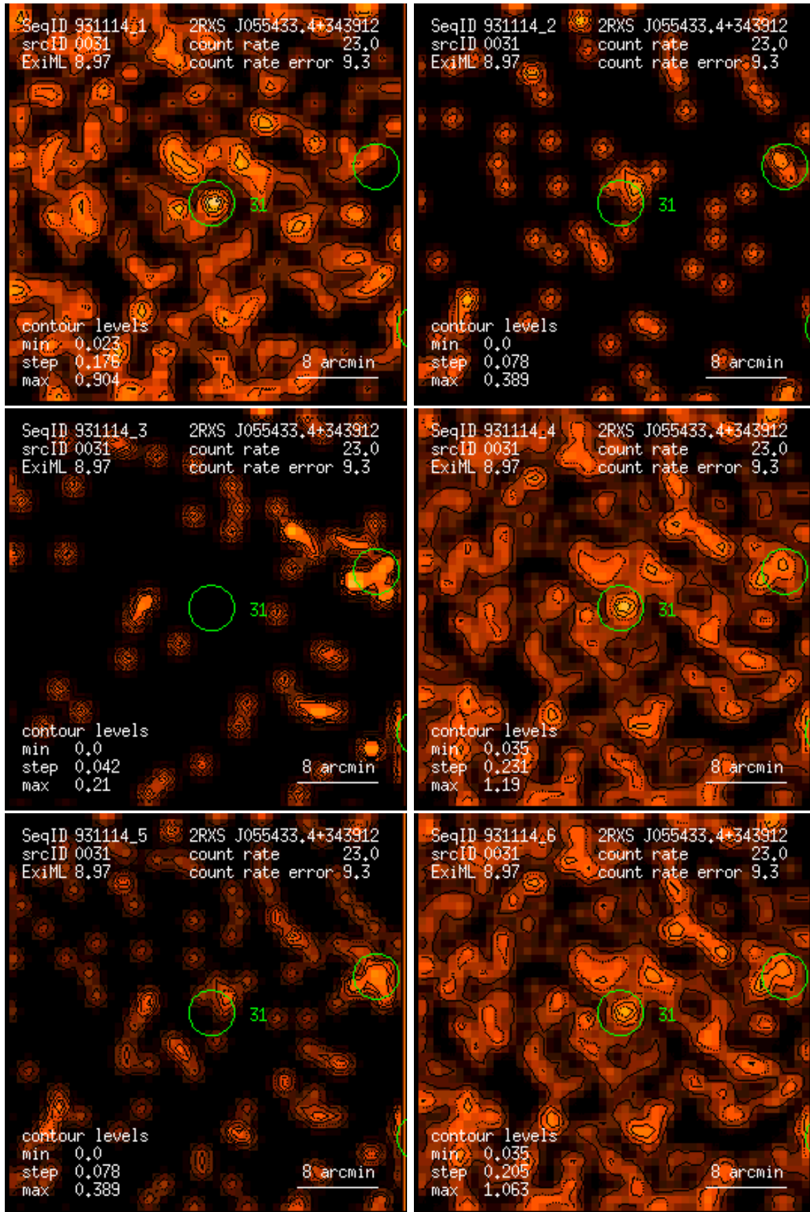
Figure 31: RASS 931114: detection 0031: band rate images, Gaussian filter: (1) PSPC channels 11 – 41, (2) 52 – 90, (3) 91 – 201, (4) 11 – 235, (5) 52 – 201, (6) 11 – 201. Broad band rates in counts/ks. Band rate contour levels in counts/ks/arcmin 2 .
