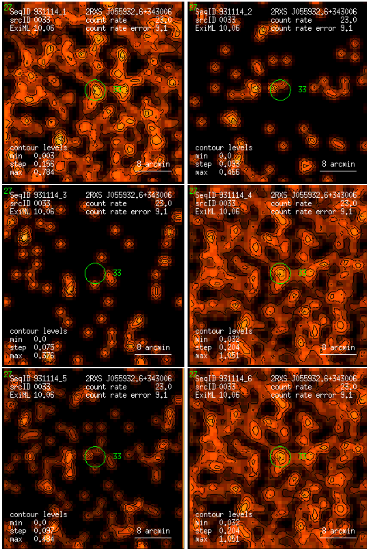
Figure 33: RASS 931114: detection 0033: band rate images, Gaussian filter: (1) PSPC channels 11 – 41, (2) 52 – 90, (3) 91 – 201, (4) 11 – 235, (5) 52 – 201, (6) 11 – 201. Broad band rates in counts/ks. Band rate contour levels in counts/ks/arcmin 2 .
