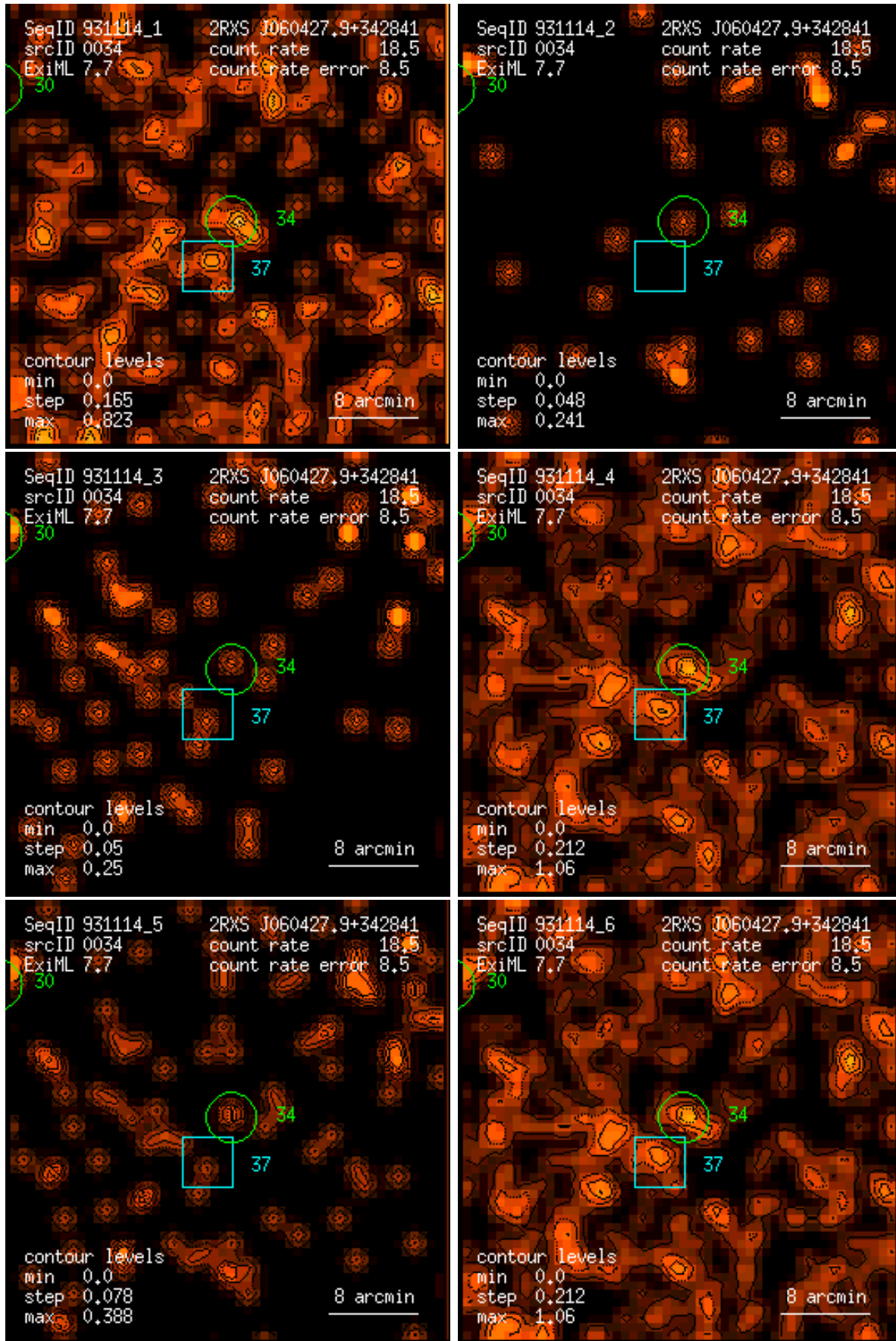
Figure 34: RASS 931114: detection 0034: band rate images, Gaussian filter: (1) PSPC channels 11 – 41, (2) 52 – 90, (3) 91 – 201, (4) 11 – 235, (5) 52 – 201, (6) 11 – 201. Broad band rates in counts/ks. Band rate contour levels in counts/ks/arcmin 2 .
