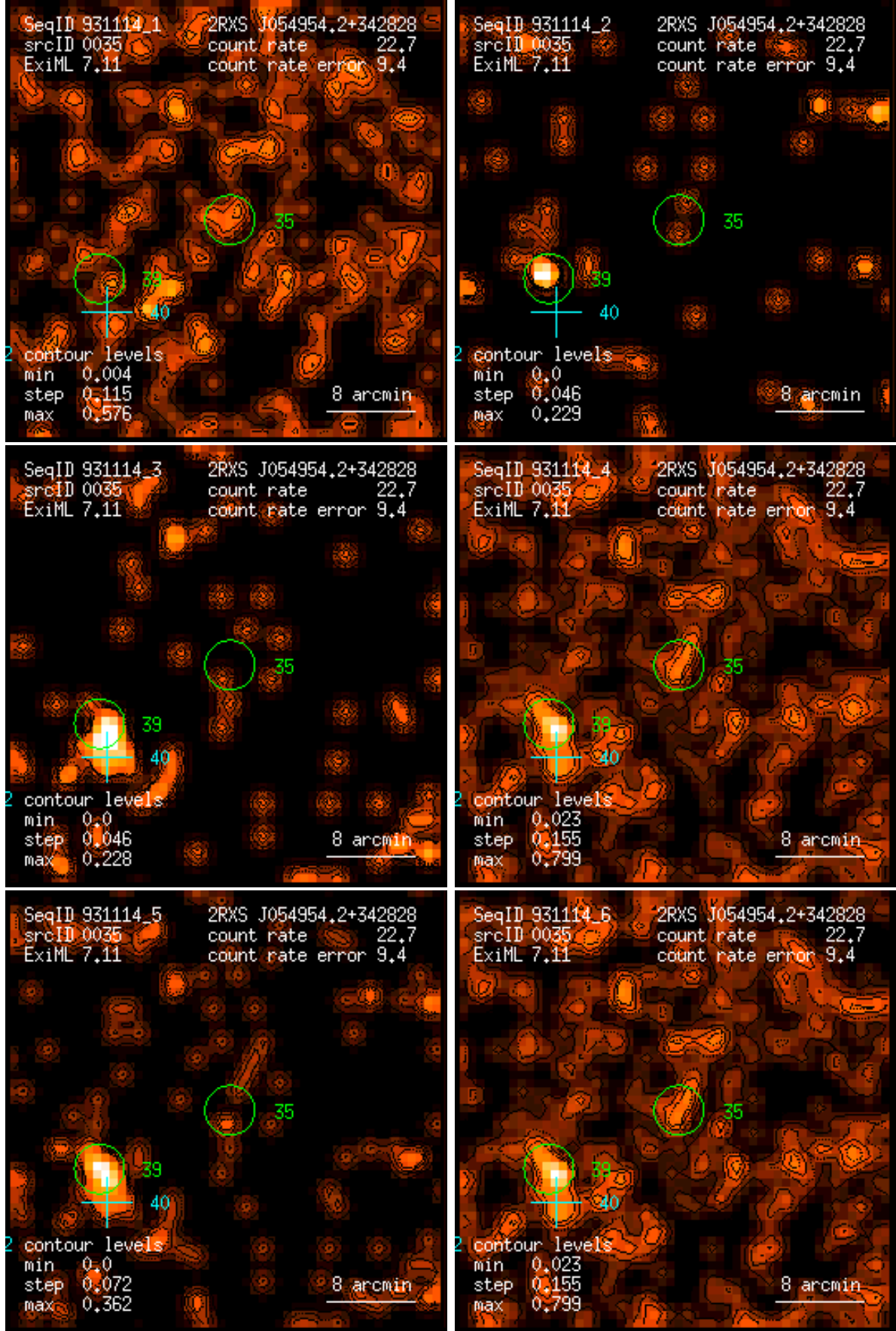
Figure 35: RASS 931114: detection 0035: band rate images, Gaussian filter: (1) PSPC channels 11 – 41, (2) 52 – 90, (3) 91 – 201, (4) 11 – 235, (5) 52 – 201, (6) 11 – 201. Broad band rates in counts/ks. Band rate contour levels in counts/ks/arcmin 2 .
