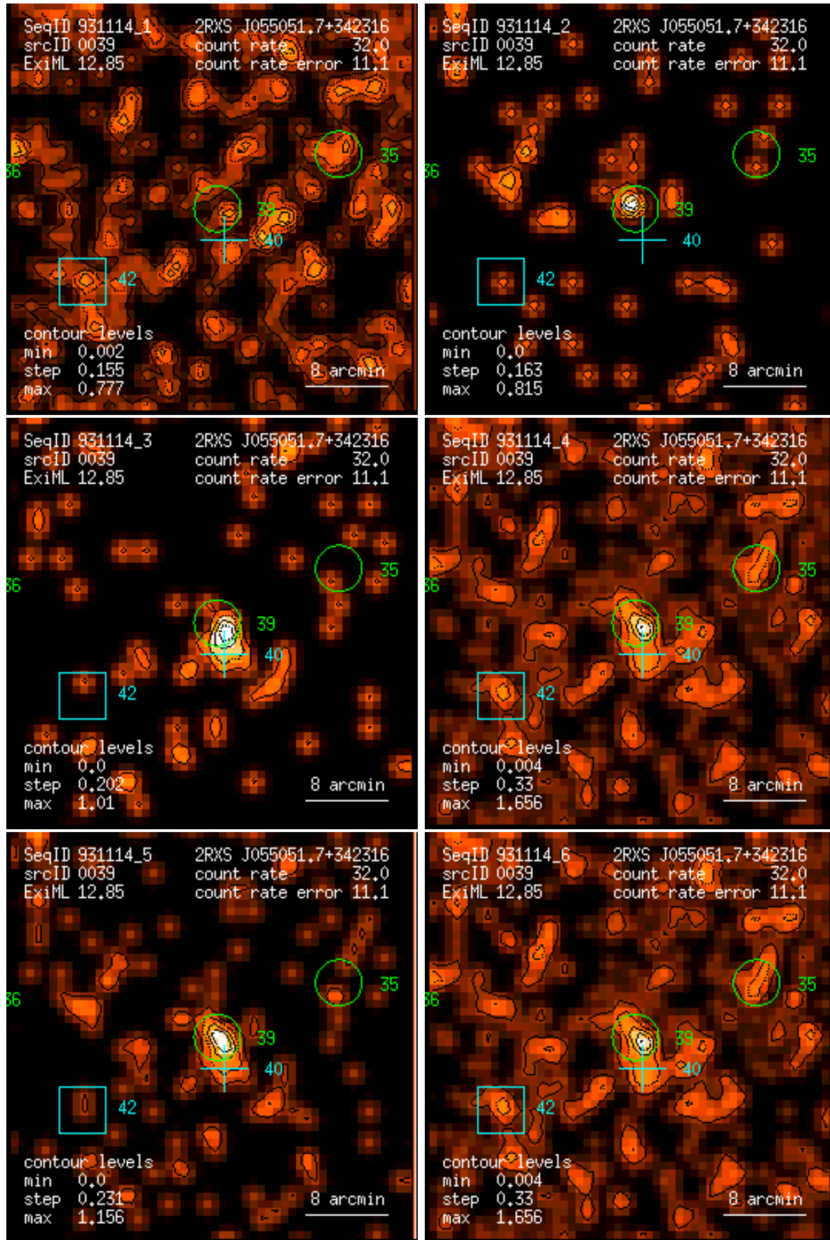
Figure 39: RASS 931114: detection 0039: band rate images, Gaussian filter: (1) PSPC channels 11 – 41, (2) 52 – 90, (3) 91 – 201, (4) 11 – 235, (5) 52 – 201, (6) 11 – 201. Broad band rates in counts/ks. Band rate contour levels in counts/ks/arcmin 2 .
