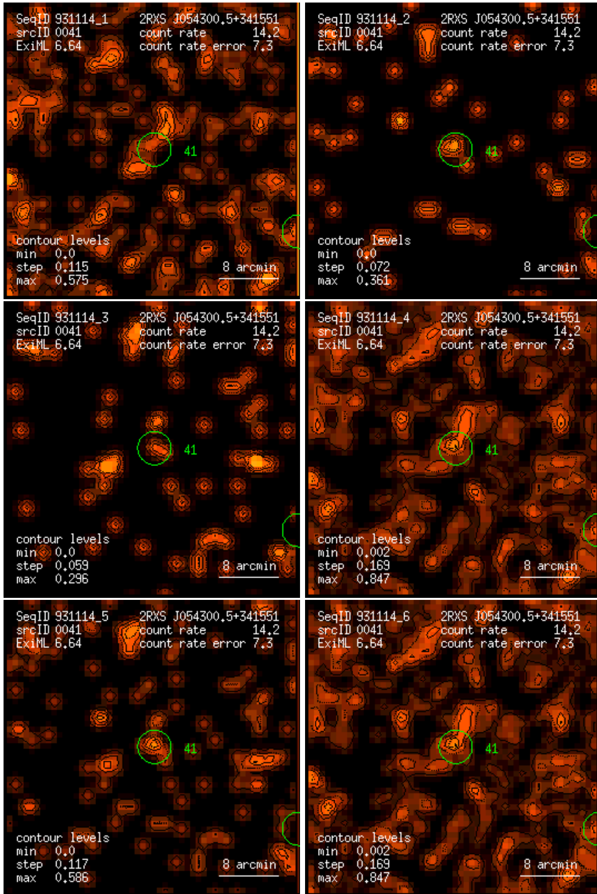
Figure 41: RASS 931114: detection 0041: band rate images, Gaussian filter: (1) PSPC channels 11 – 41, (2) 52 – 90, (3) 91 – 201, (4) 11 – 235, (5) 52 – 201, (6) 11 – 201. Broad band rates in counts/ks. Band rate contour levels in counts/ks/arcmin 2 .
