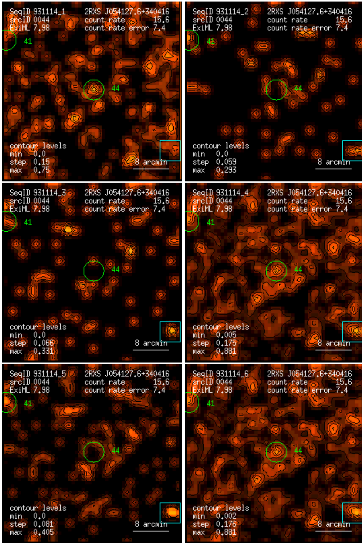
Figure 44: RASS 931114: detection 0044: band rate images, Gaussian filter: (1) PSPC channels 11 – 41, (2) 52 – 90, (3) 91 – 201, (4) 11 – 235, (5) 52 – 201, (6) 11 – 201. Broad band rates in counts/ks. Band rate contour levels in counts/ks/arcmin 2 .
