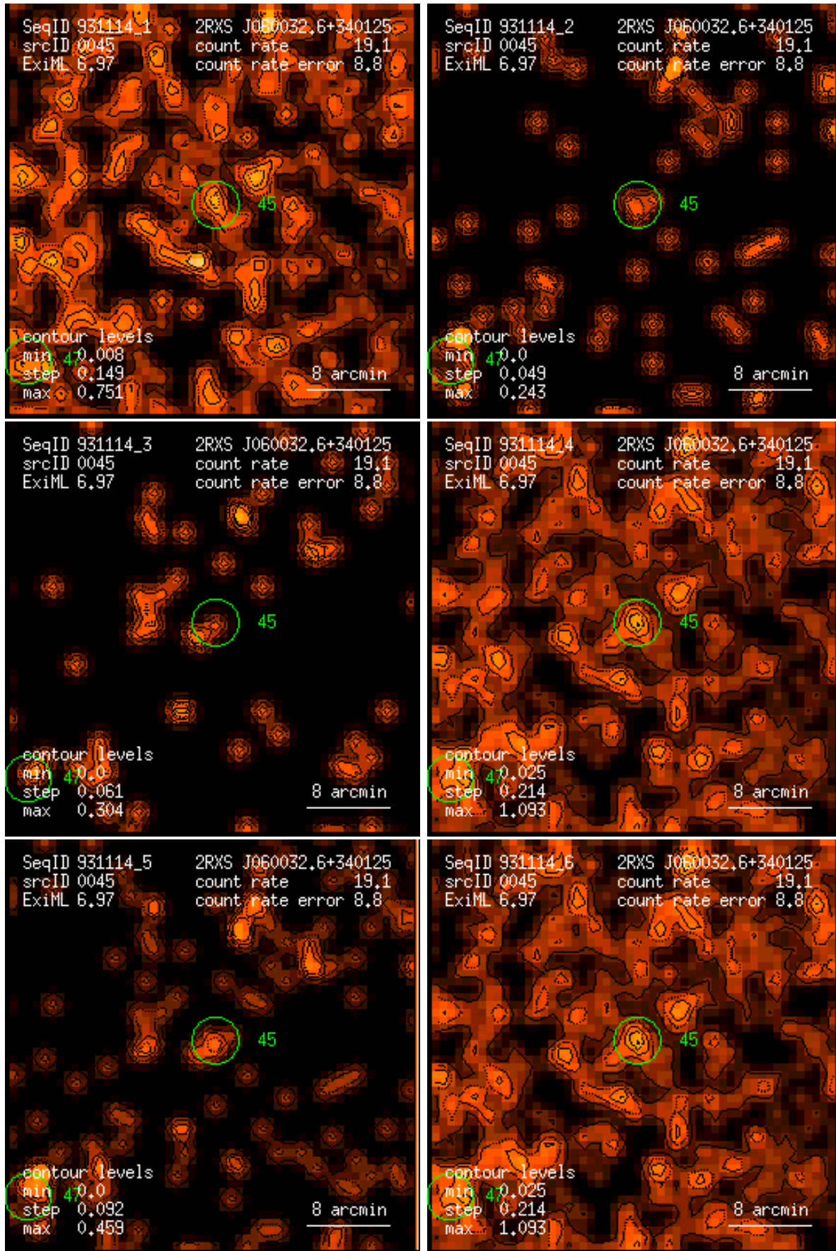
Figure 45: RASS 931114: detection 0045: band rate images, Gaussian filter: (1) PSPC channels 11 – 41, (2) 52 – 90, (3) 91 – 201, (4) 11 – 235, (5) 52 – 201, (6) 11 – 201. Broad band rates in counts/ks. Band rate contour levels in counts/ks/arcmin 2 .
