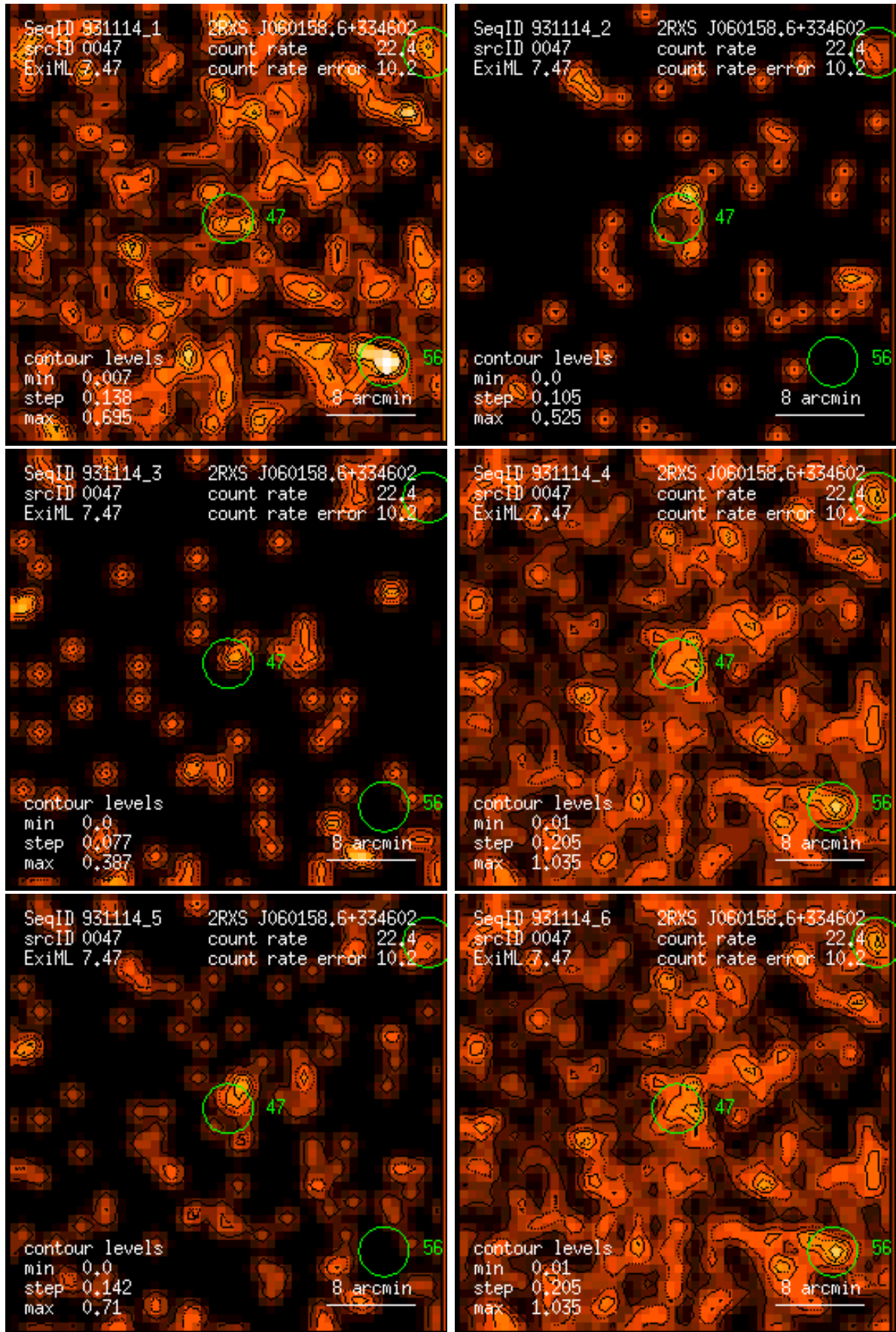
Figure 47: RASS 931114: detection 0047: band rate images, Gaussian filter: (1) PSPC channels 11 – 41, (2) 52 – 90, (3) 91 – 201, (4) 11 – 235, (5) 52 – 201, (6) 11 – 201. Broad band rates in counts/ks. Band rate contour levels in counts/ks/arcmin 2 .
